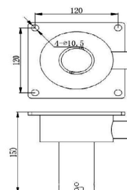
Bracket for Wall or Ceiling
