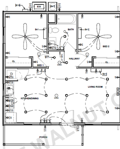
1 ELECTRICAL PLAN A1-201 A4-111 SCALE: 1/4" = 1'-0"
