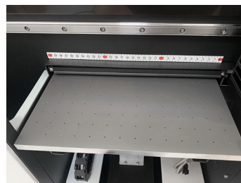
High precision suction platform (within 0.1mm flatness)
