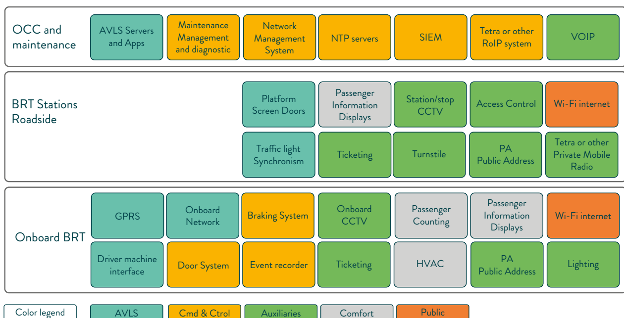
Figure 23: Example of Generic BRT asset model; Source: Serge Van Themsche adapted from TS 50701
