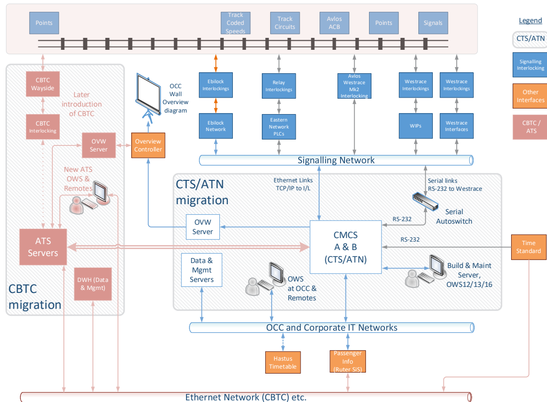
Figure 34: Example of a CBTC architecture explaining the functional interface; Source: Sporveien tender documents
