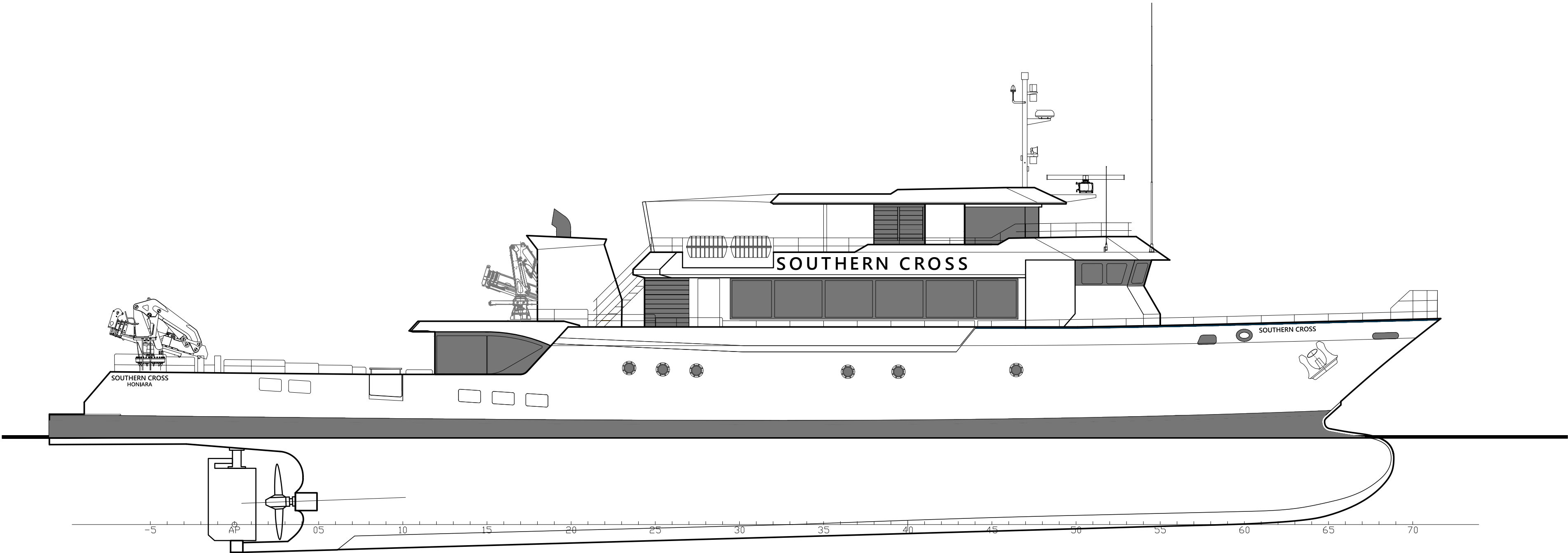
OUTBOARD PROFILE
