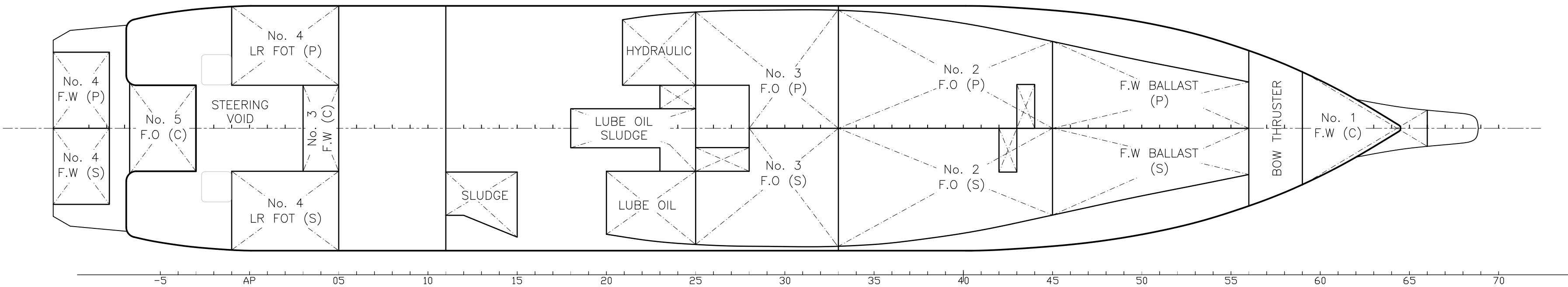
TANK PLAN
