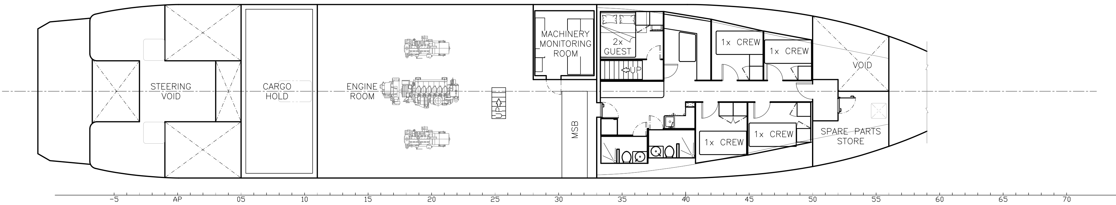
LOWER DECK
