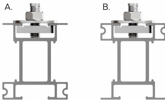
Nexus Profile installation for metal tile
