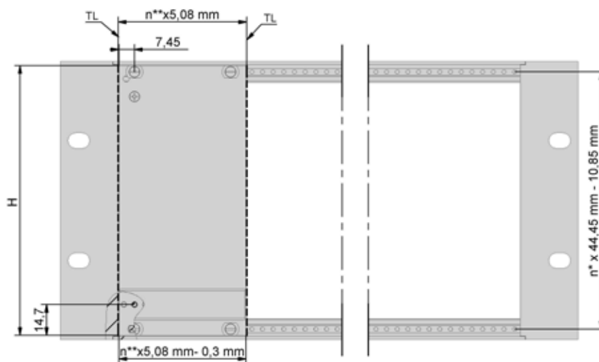
Mounting dimensions (mm)
