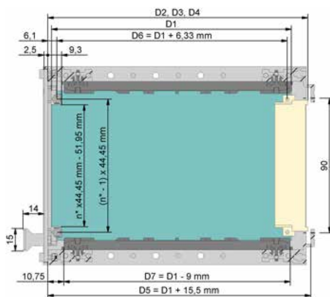
Dimensions for plug-in modules (mm)
