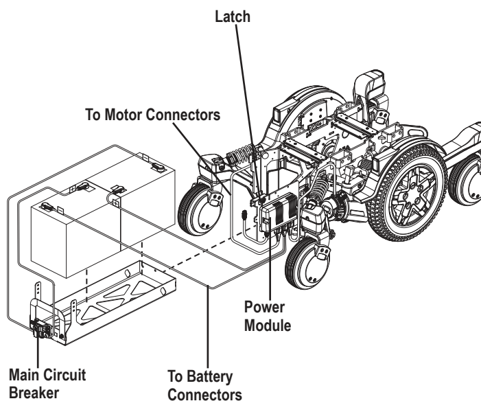
Figure 1. Electrical Components
