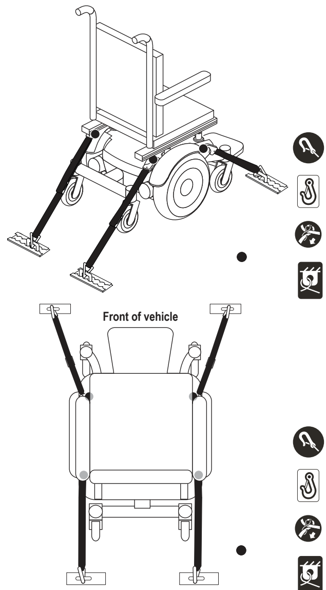
Figure 6. Unoccupied Transit System Securement Points
