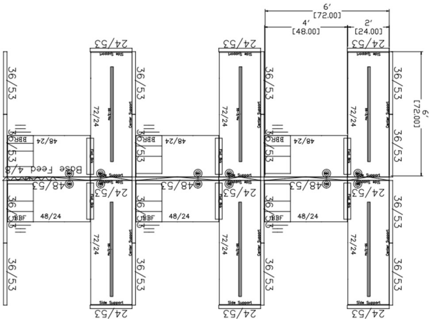
2D PLAN LAYOUT
