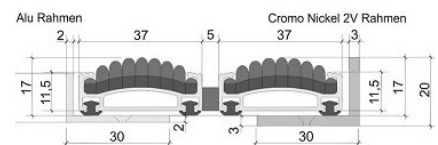
Alumatte Robust - Rips Höhe 17 mm
