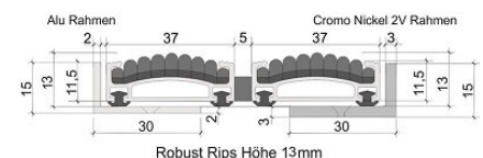
Alumatte Robust - Rips Höhe 13 mm
