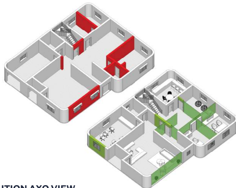
DEMOLITION AXO VIEW
