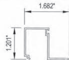
12 GLAZING BEAD FOR 9/16" GLASS DIE # 1060-008 MATERIAL: ALUMINUM ALLOY: 6063-T6 TYPICAL WALL: .050"
