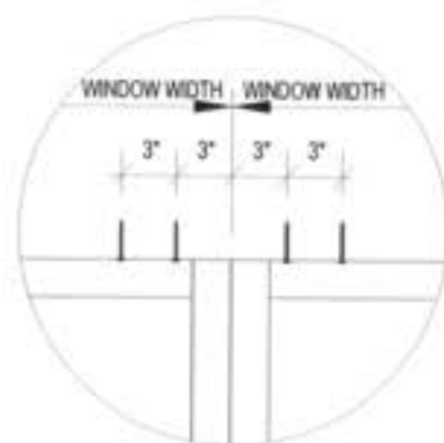
DETAIL "A" TYPICAL CLUSTER OF ANCHORS AT INTERLOCKS TOP & BOTTOM (ONLY AT UNCLIPPED MULLION CONDITIONS)
