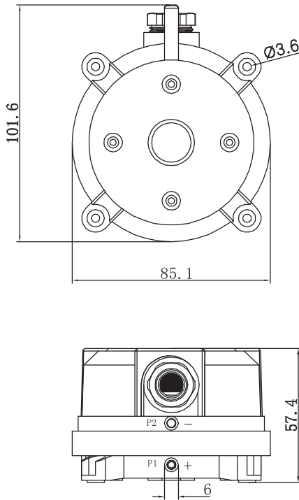
Dimension in:mm
