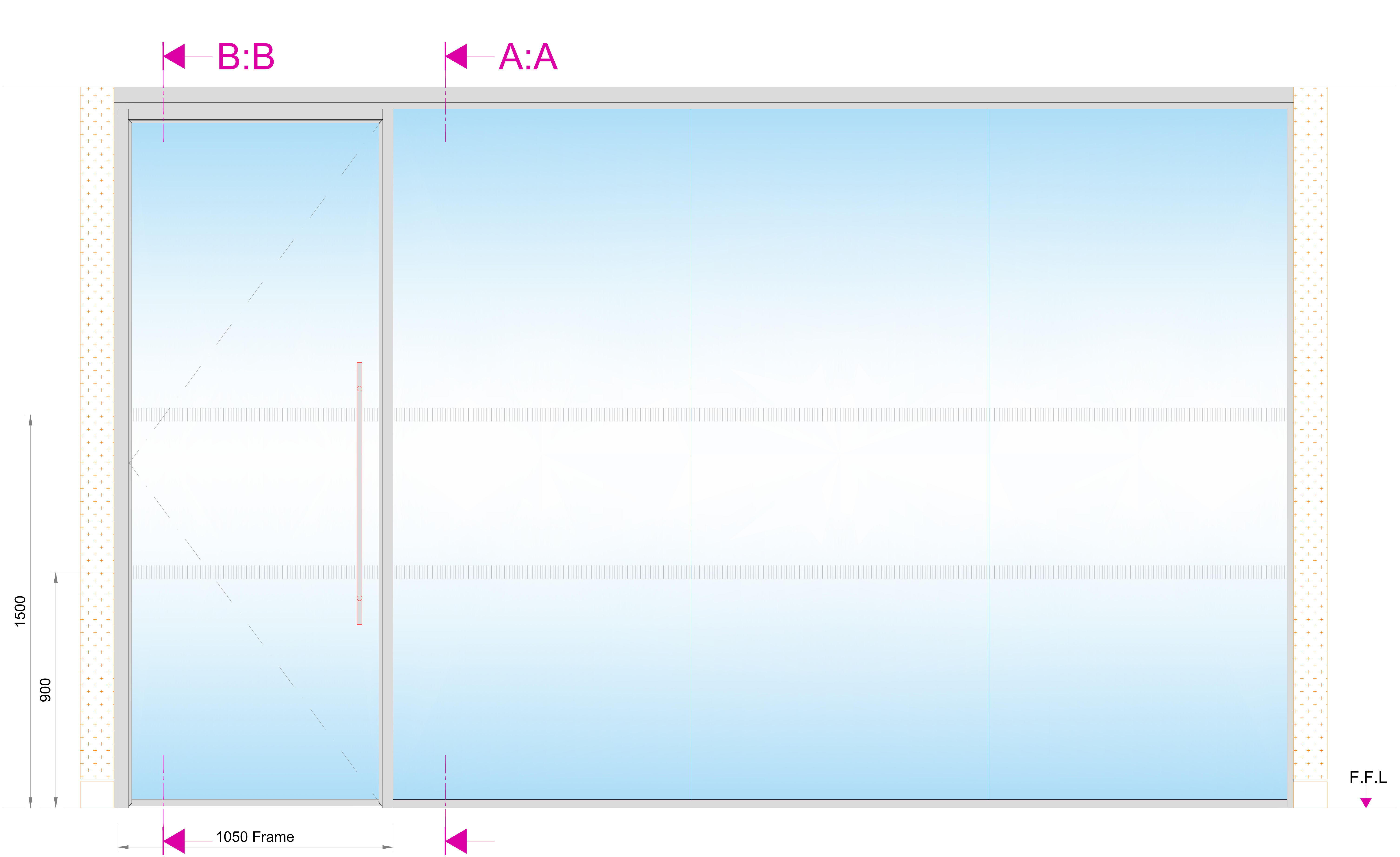
ELEVATION SILENCE 50 Single Glazing with FULCRA Single Glazed Pivot Door
