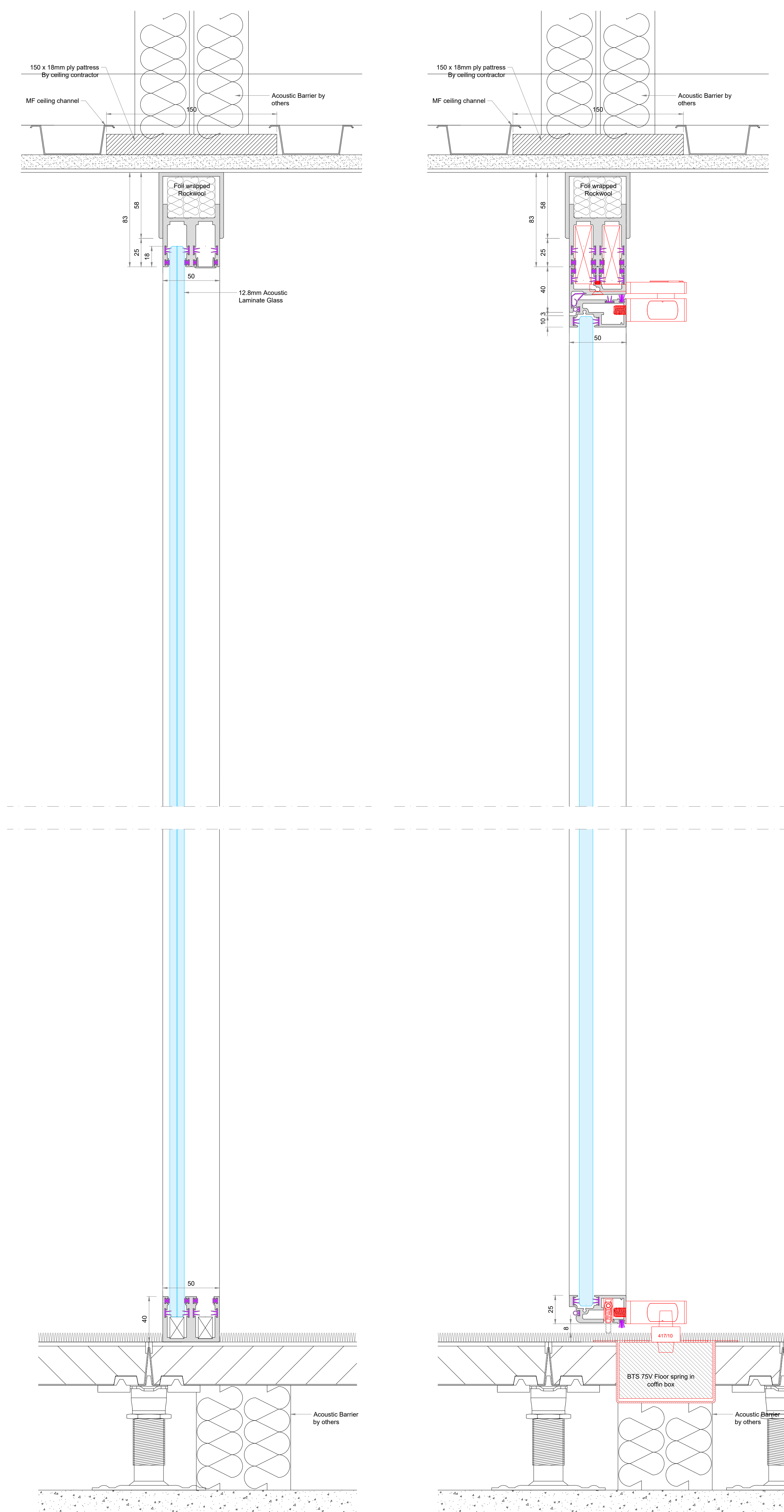
VERTICAL SECTION A:A SILENCE 50 Single Glazing +/- 25mm Deflection Scale 1:2 @ A0 Acoustic Integrity: 39dB Rw
