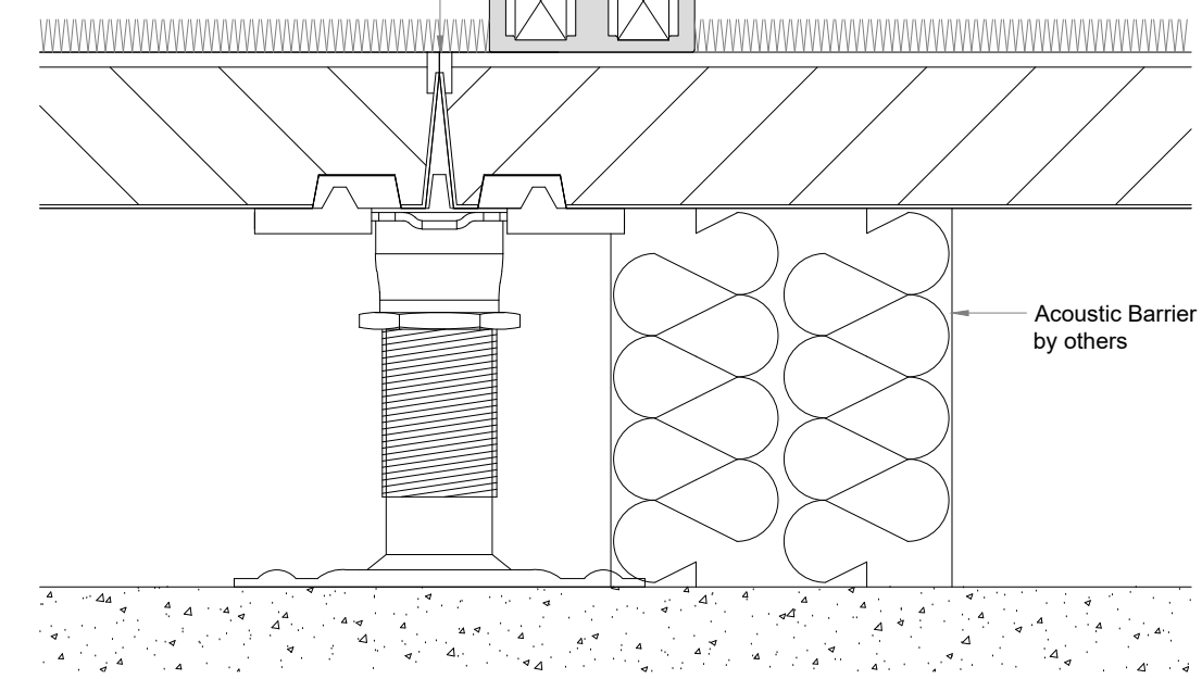
VERTICAL SECTION A:A SILENCE 50 Single Glazing +/- 25mm Deflection Scale 1:2 @ A0 Acoustic Integrity: 39dB Rw
