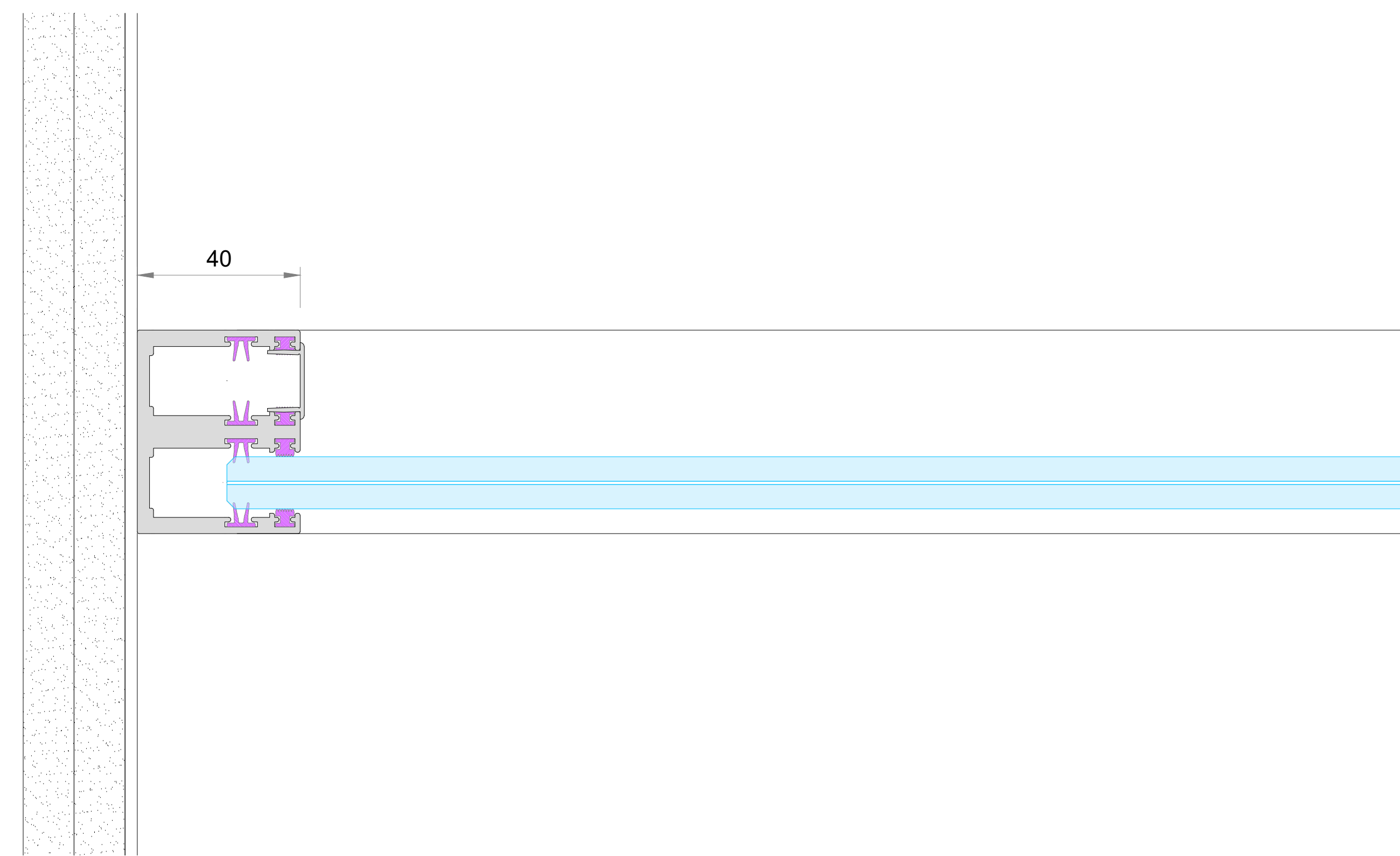
OPTION 2 40mm Abutment
