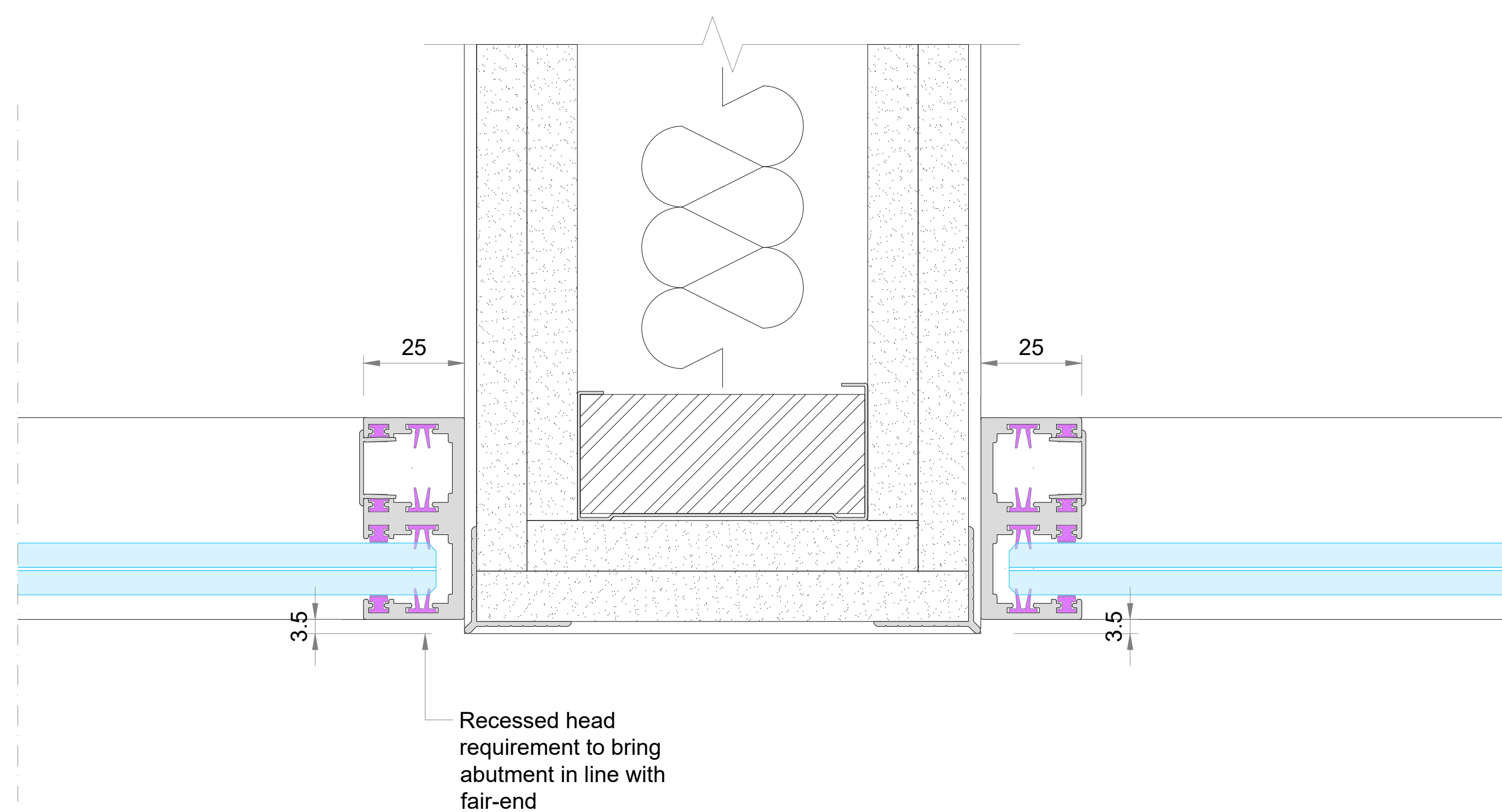
3-WAY OPTION 1 Drywall FairEnds to Break Systems
