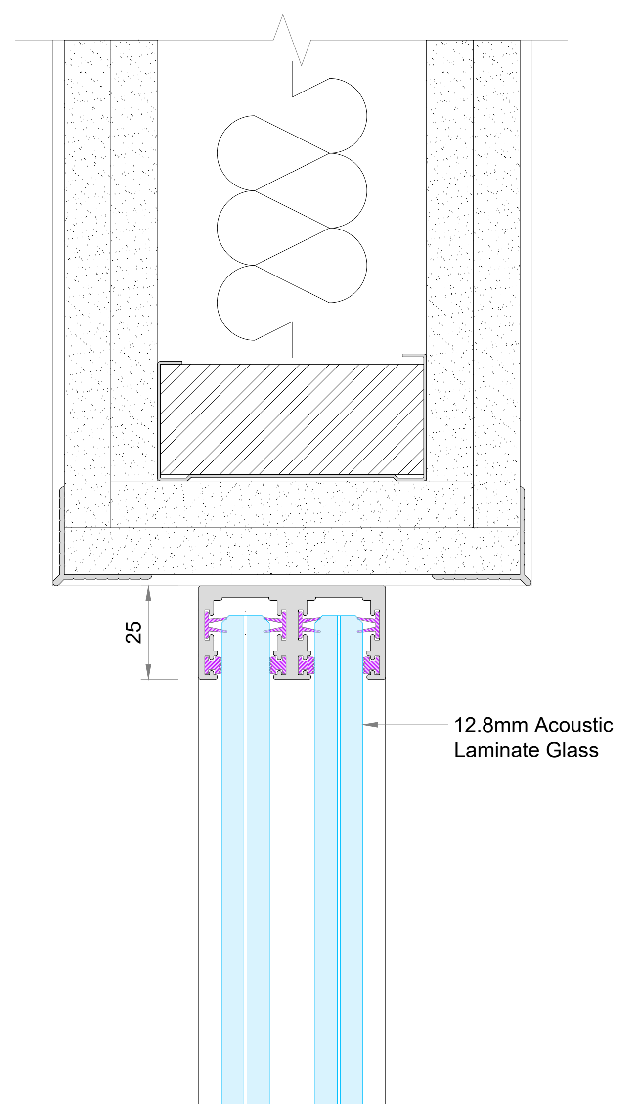
FAIREND ABUTMENT OPTION 1 Surface Mounted Abutment to Drywall Fairend
