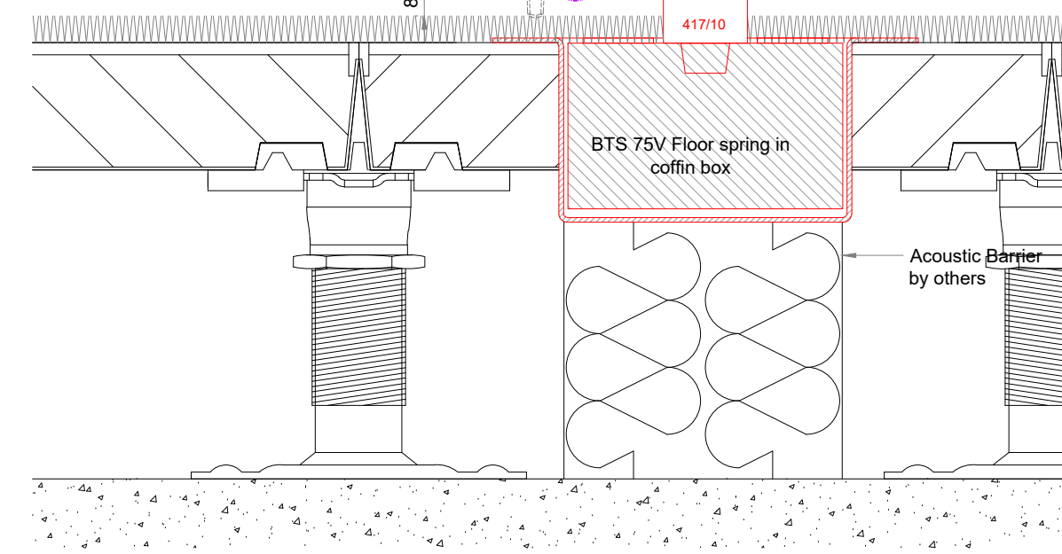
VERTICAL SECTION B:B FULCRA Single Glazed Pivot Door +/- 25mm Deflection Scale 1:2 @ A0 Acoustic Integrity: 34dB Rw
