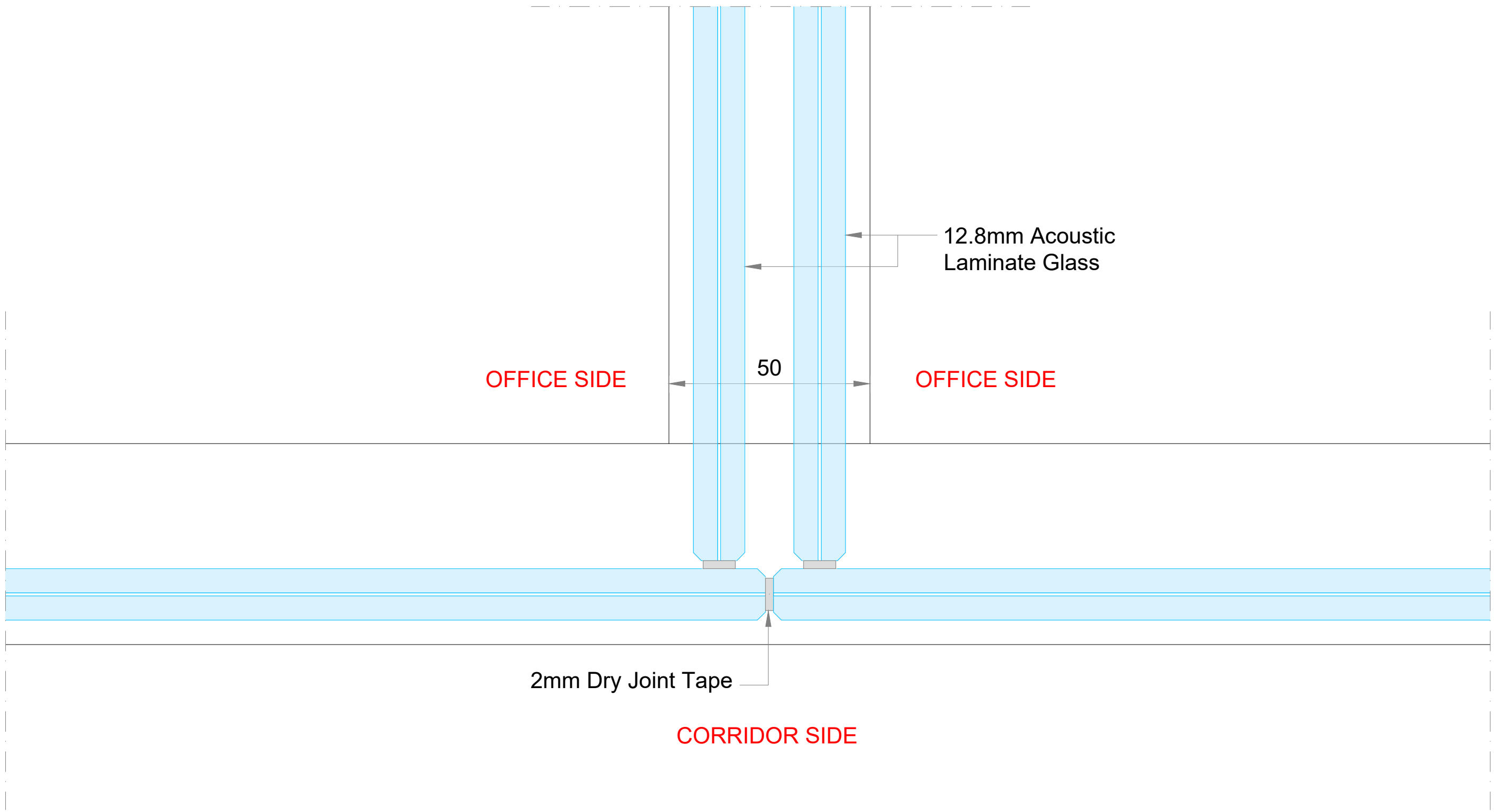
3-WAY OPTION 2 Silence 50 Return Fin Acoustic Integrity: 45dB Rw
