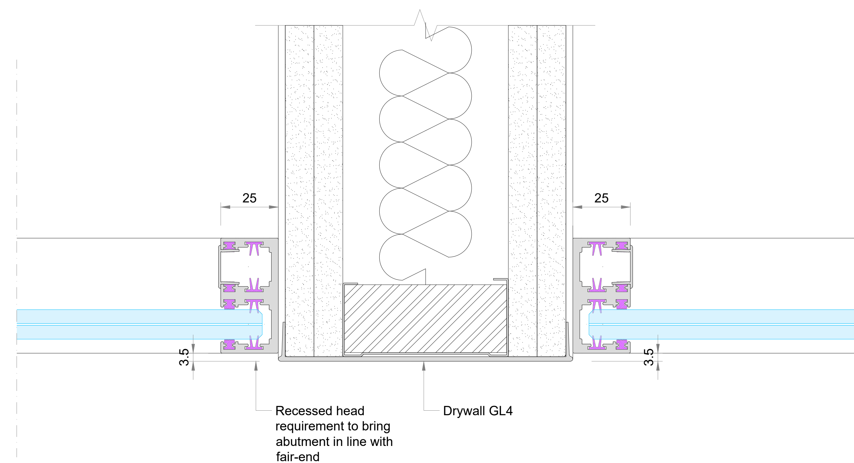
3-WAY OPTION 2 Drywall GL4 Endcap to Break Systems
