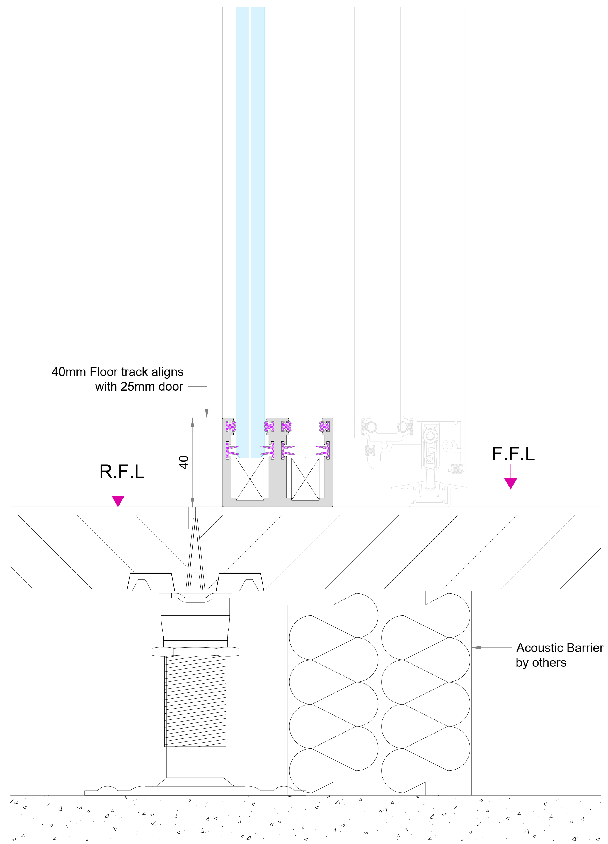
OPTION 2 40mm Base Track
