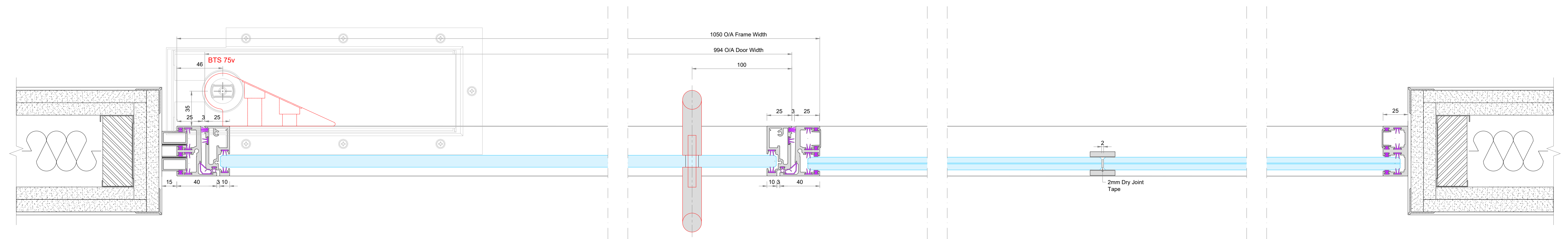
HORIZONTAL SECTION SILENCE 50 Single Glazing with FULCRA Single Glazed Pivot Door Scale 1:2@A0
