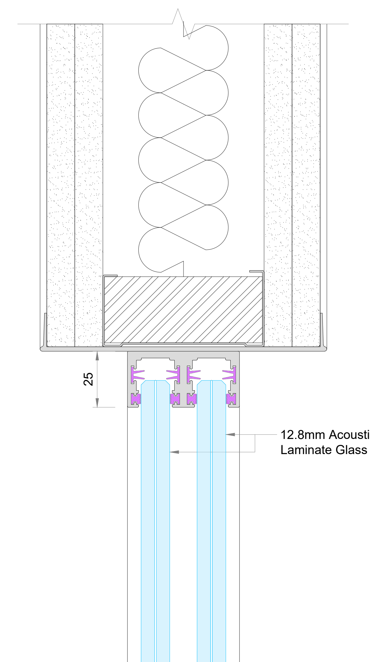
FAIREND ABUTMENT OPTION 2 Surface Mounted Abutment to Drywall Endcap
