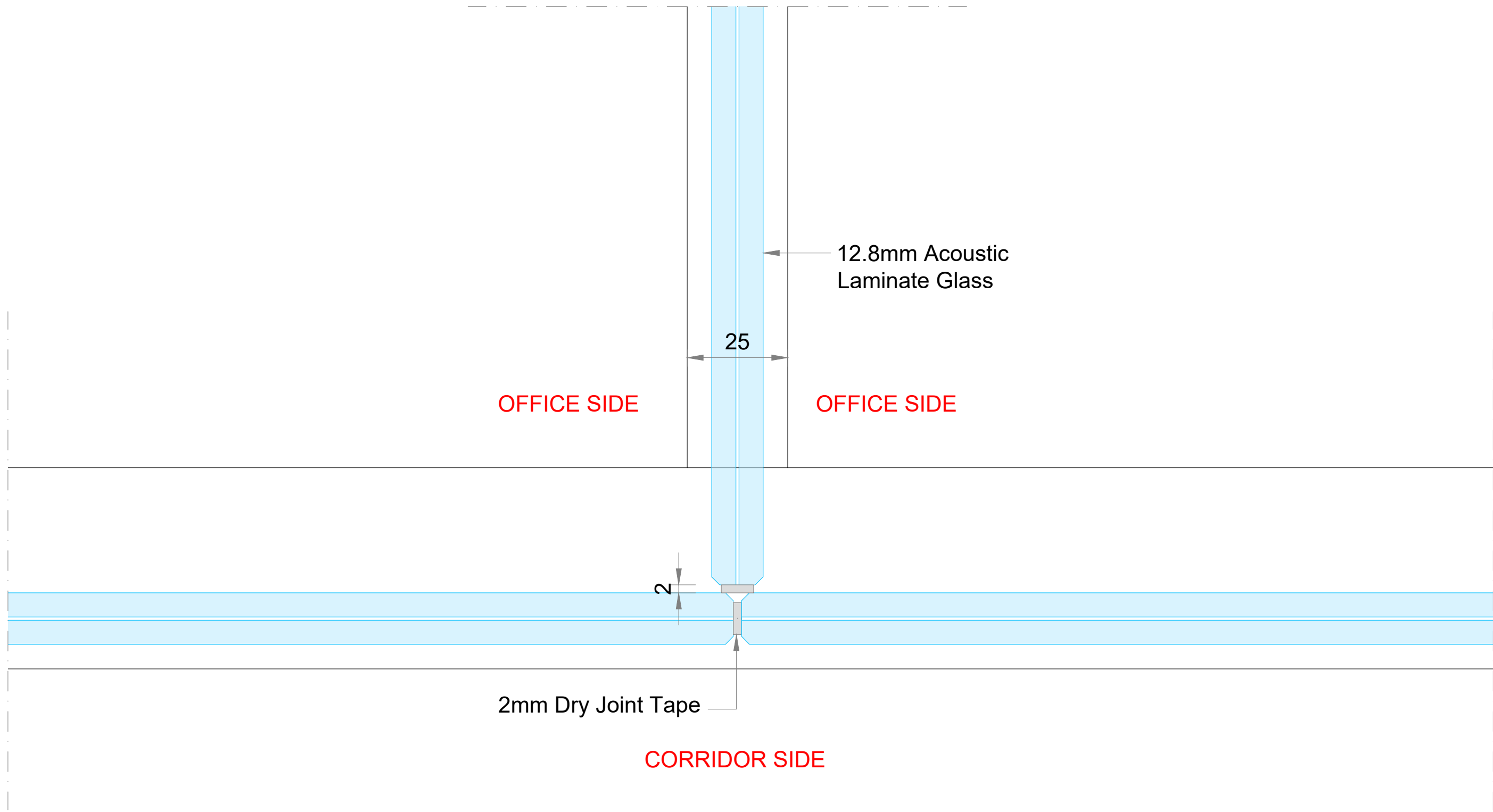
3-WAY OPTION 1 Silence 25 Return Fin Acoustic Integrity: 38dB Rw
