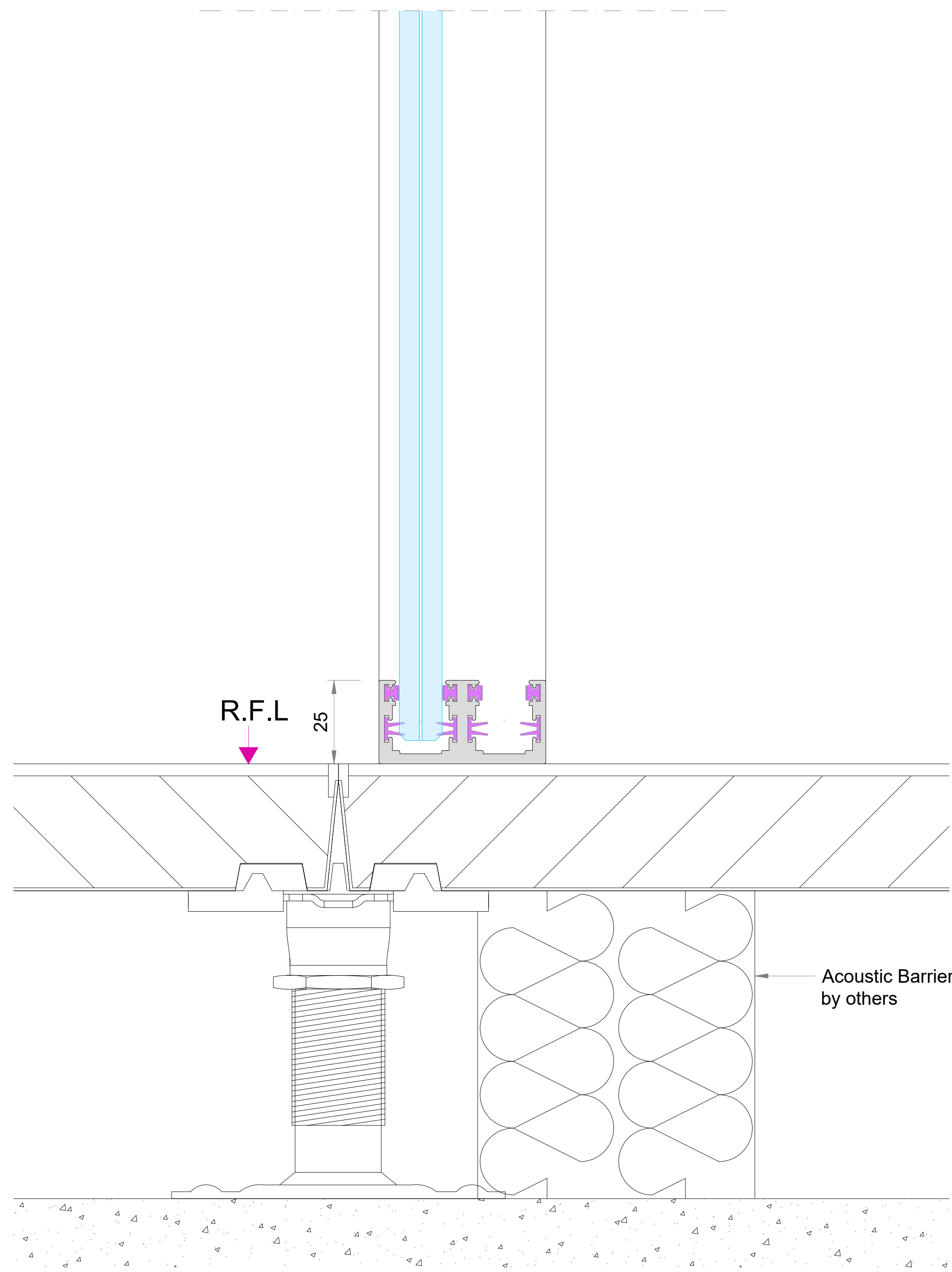
OPTION 1 25mm Base Track
