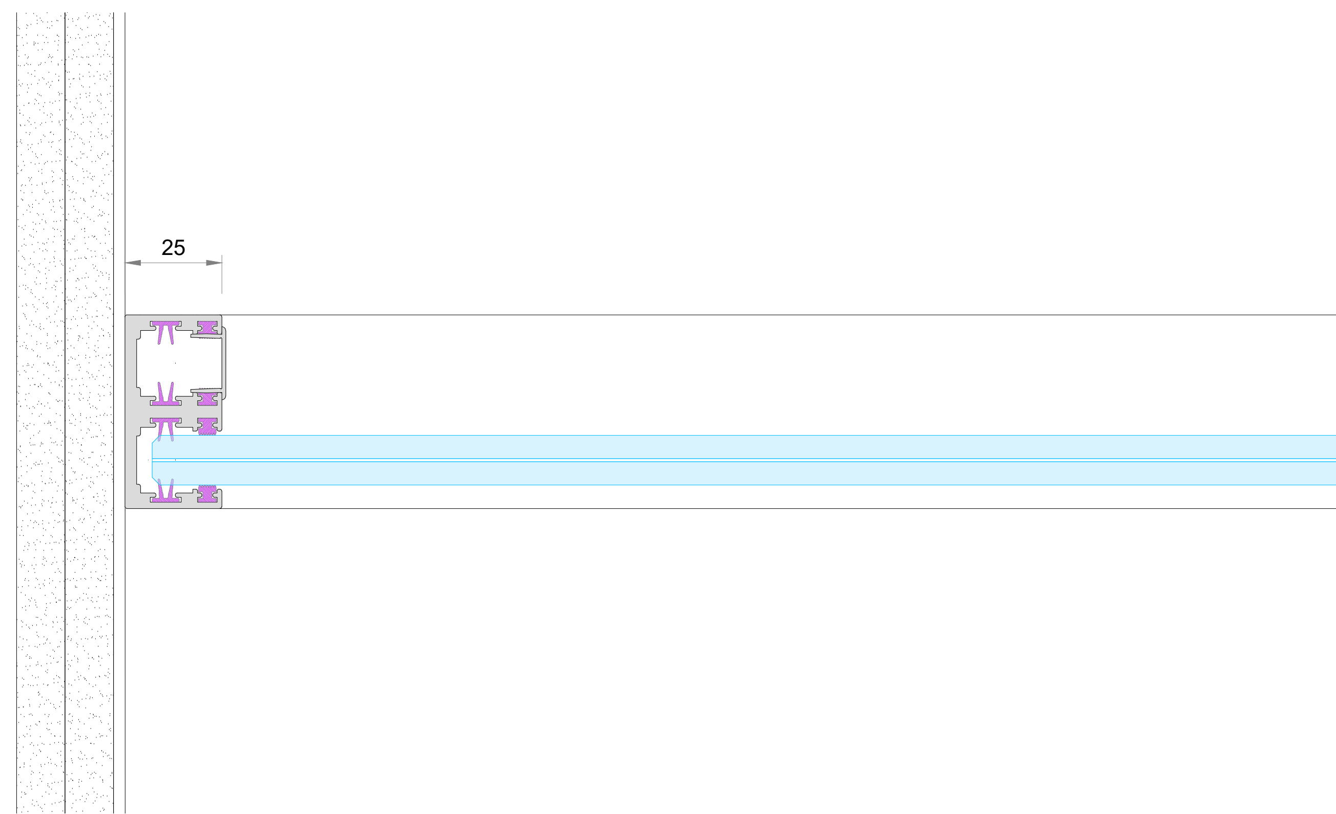
OPTION 1 25mm Abutment
