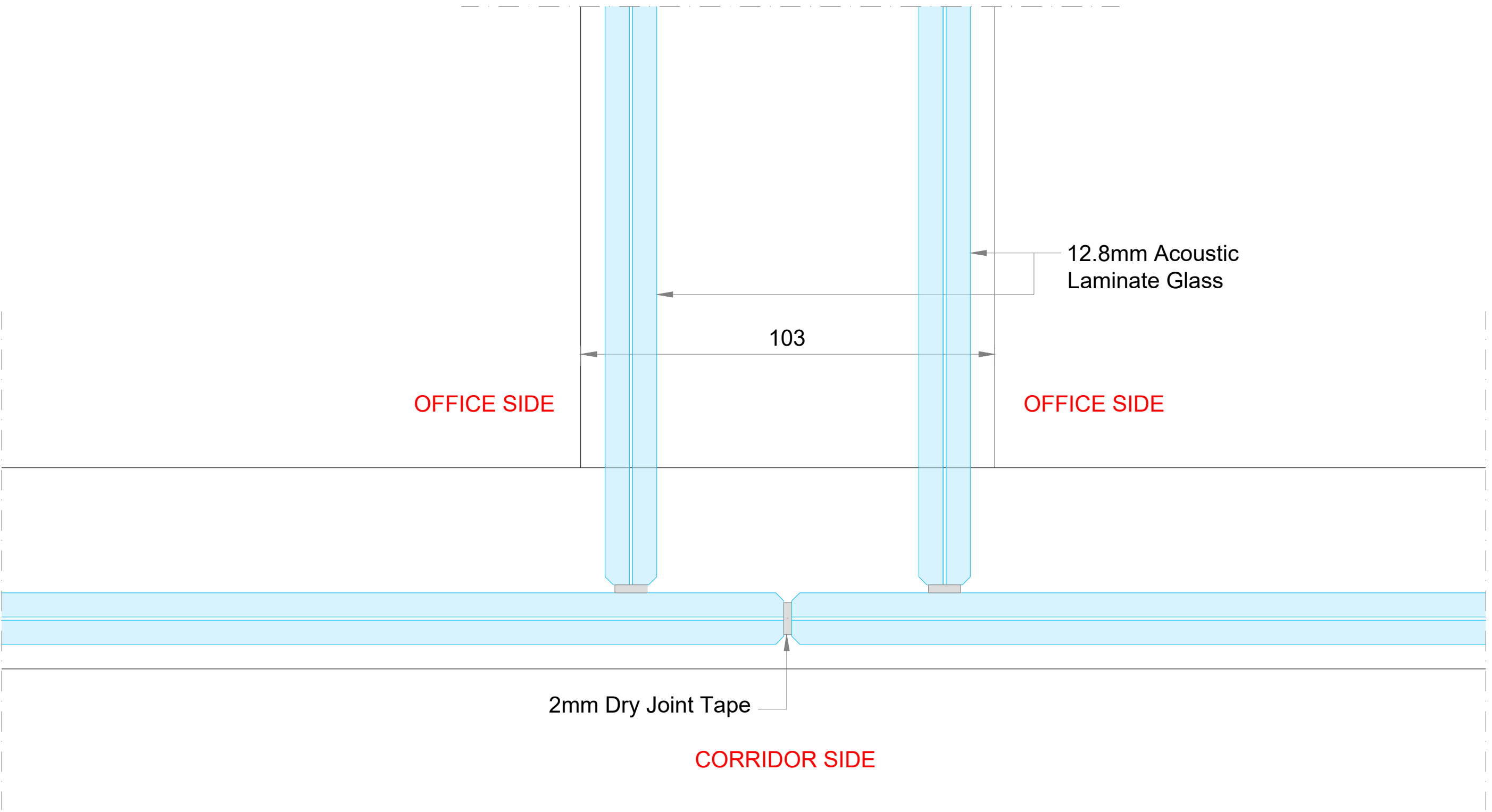
3-WAY OPTION 3 Silence 100 Return Fin Acoustic Integrity: 50dB Rw
