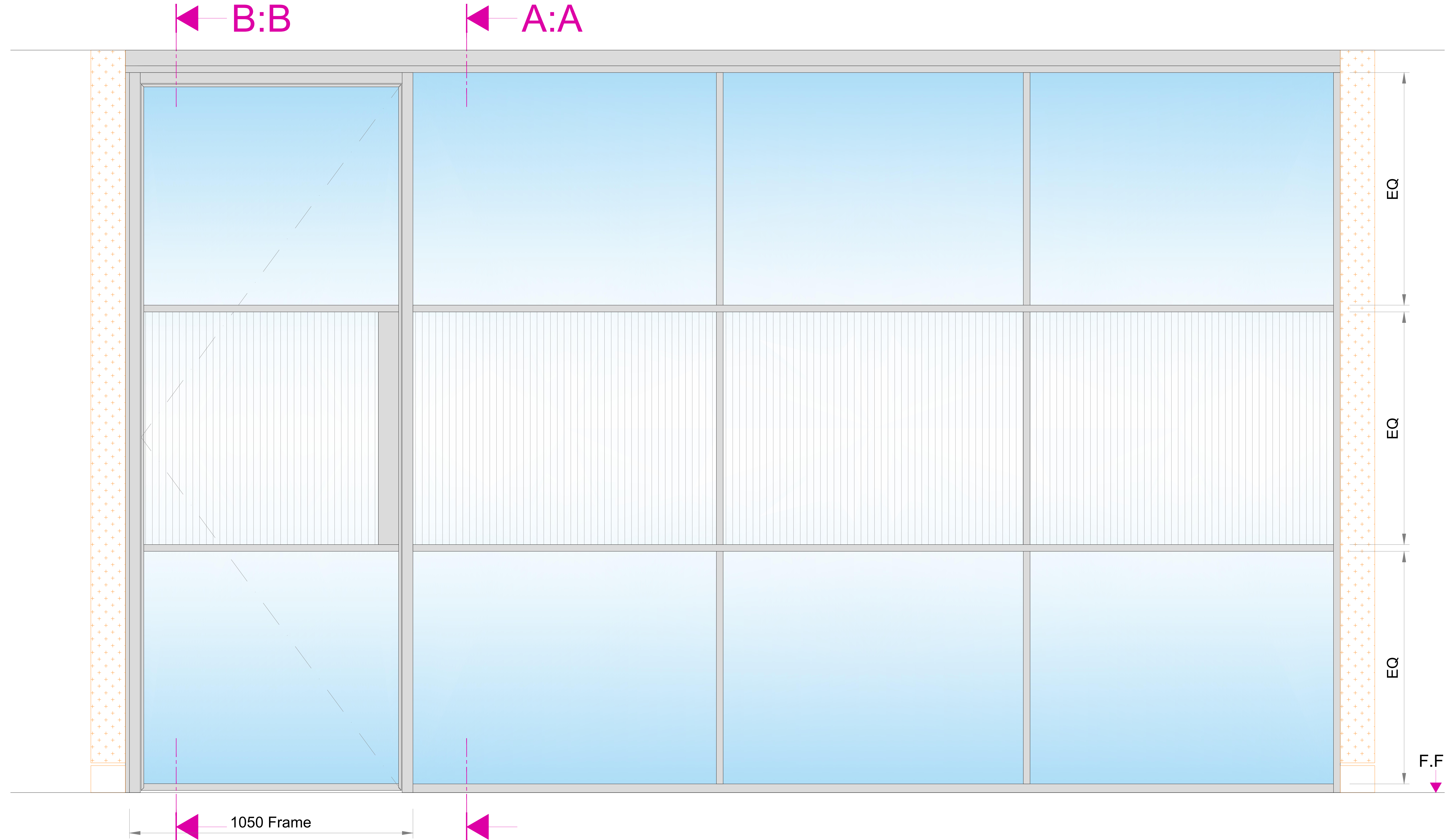
ELEVATION SILENCE 50 Single Glazing with FULCRA Single Glazed Pivot Door
