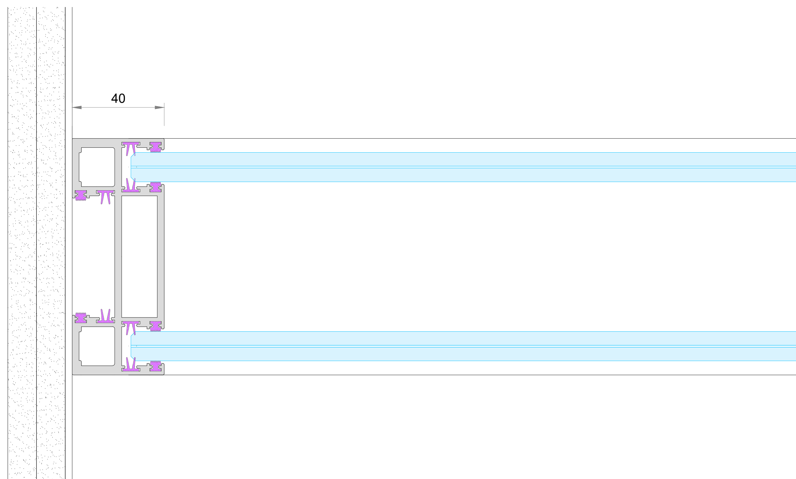
OPTION 1 40mm Abutment
