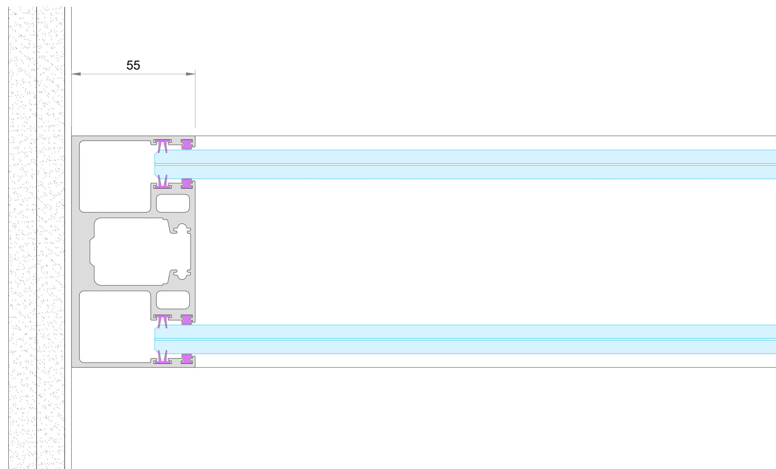
OPTION 2 55mm Abutment
