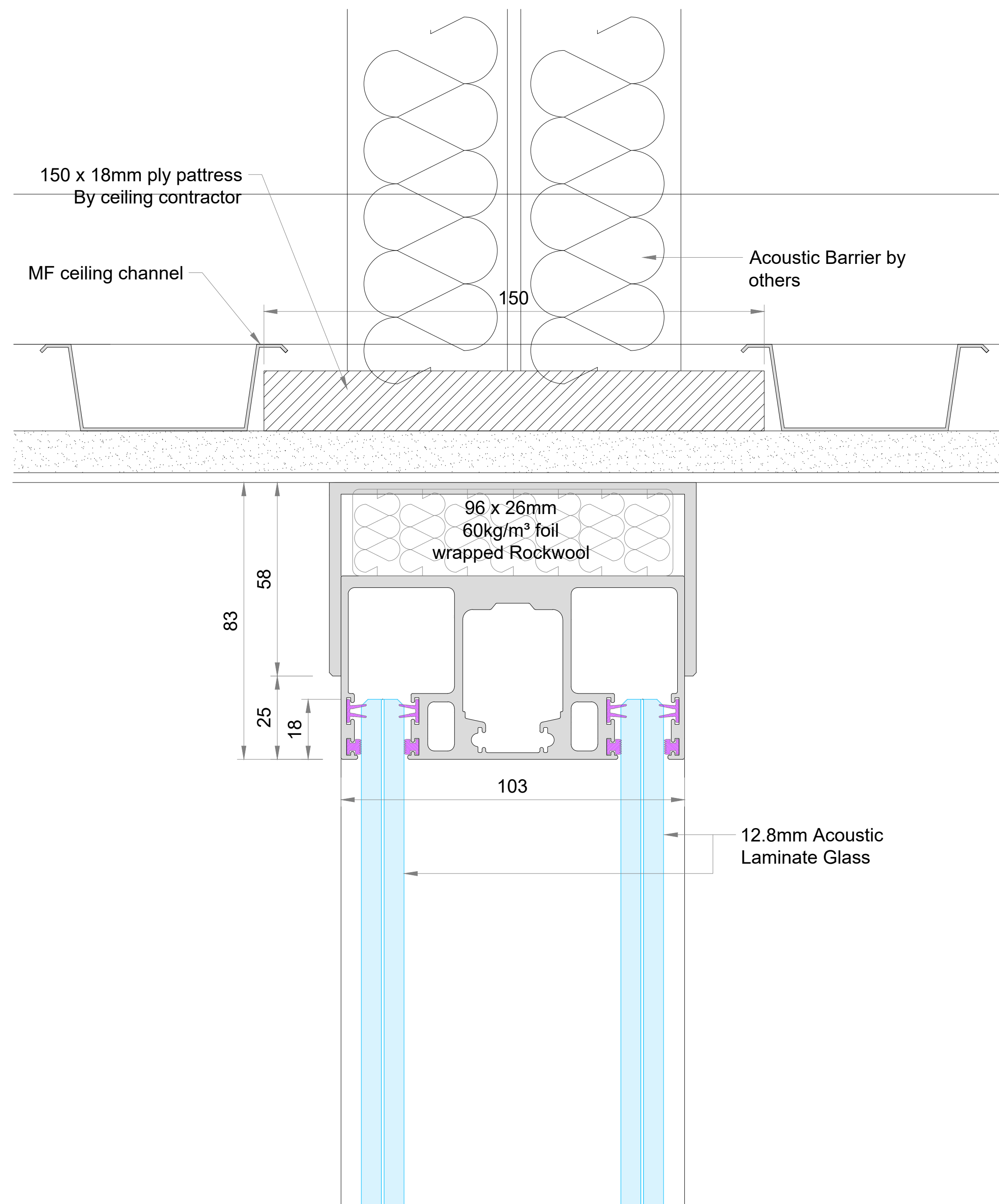
OPTION 1 Surface Mounted Deflection +/- 25mm
