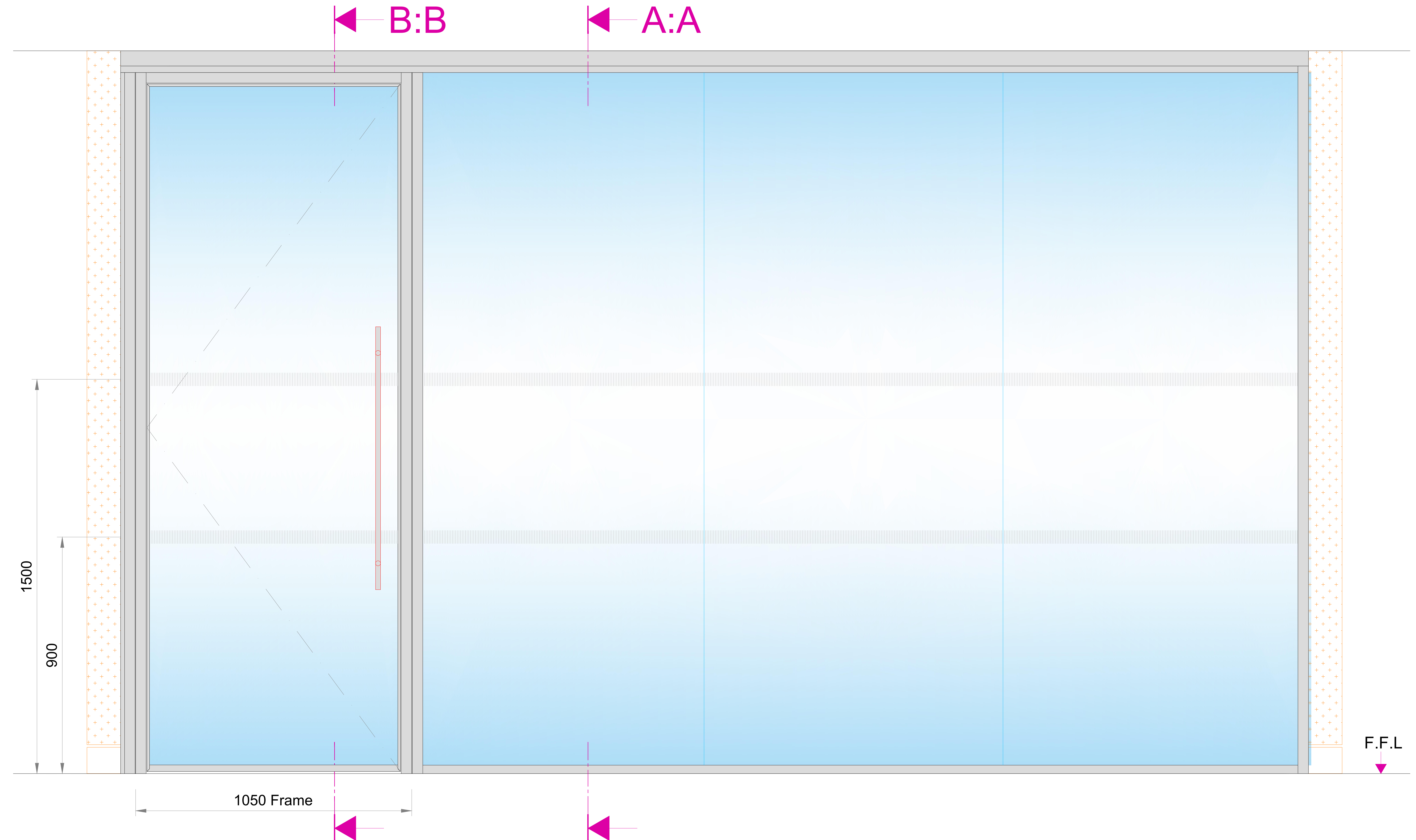
ELEVATION SILENCE 100 Double Glazing with FULCRUM Single Glazed Pivot Door
