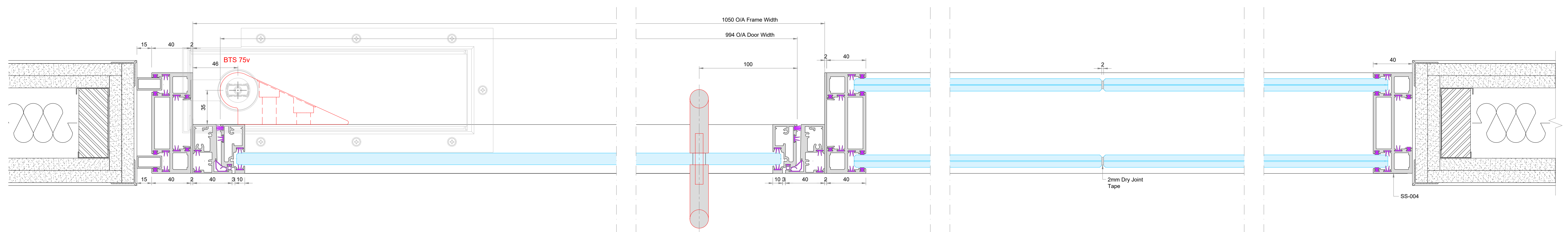
HORIZONTAL SECTION SILENCE 100 Double Glazing with FULCRUM Single Glazed Pivot Door Scale 1:2@A0
