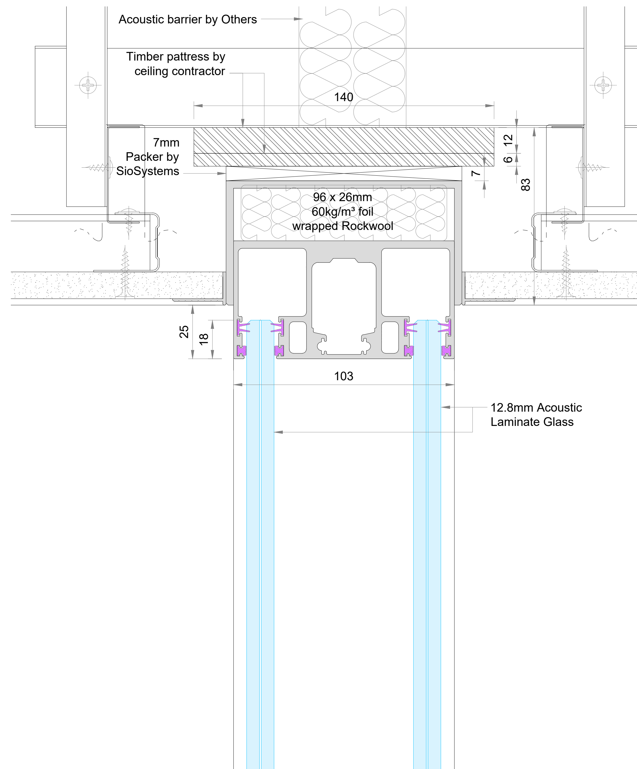
OPTION 2 Recessed Deflection in Ceiling +/- 25mm
