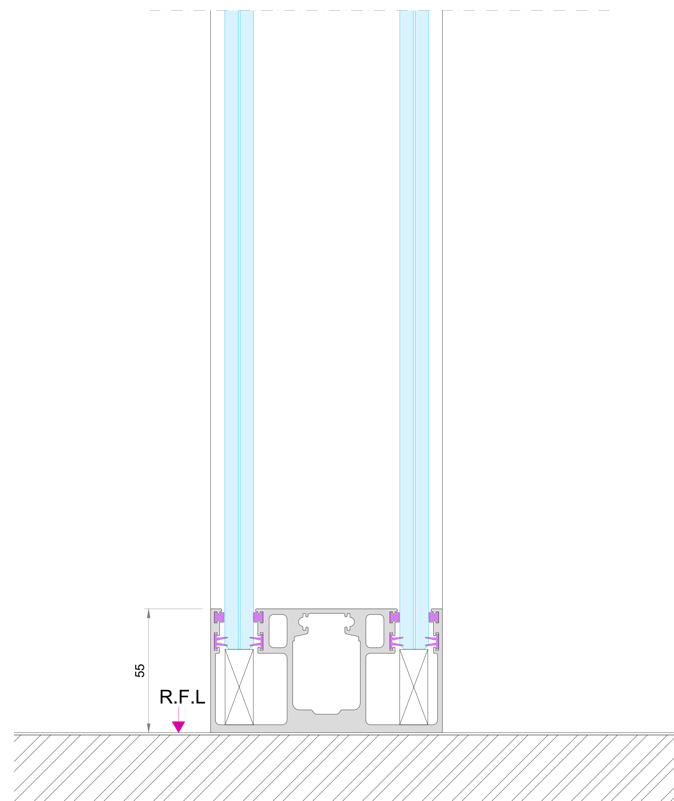
OPTION 2 55mm Base Track
