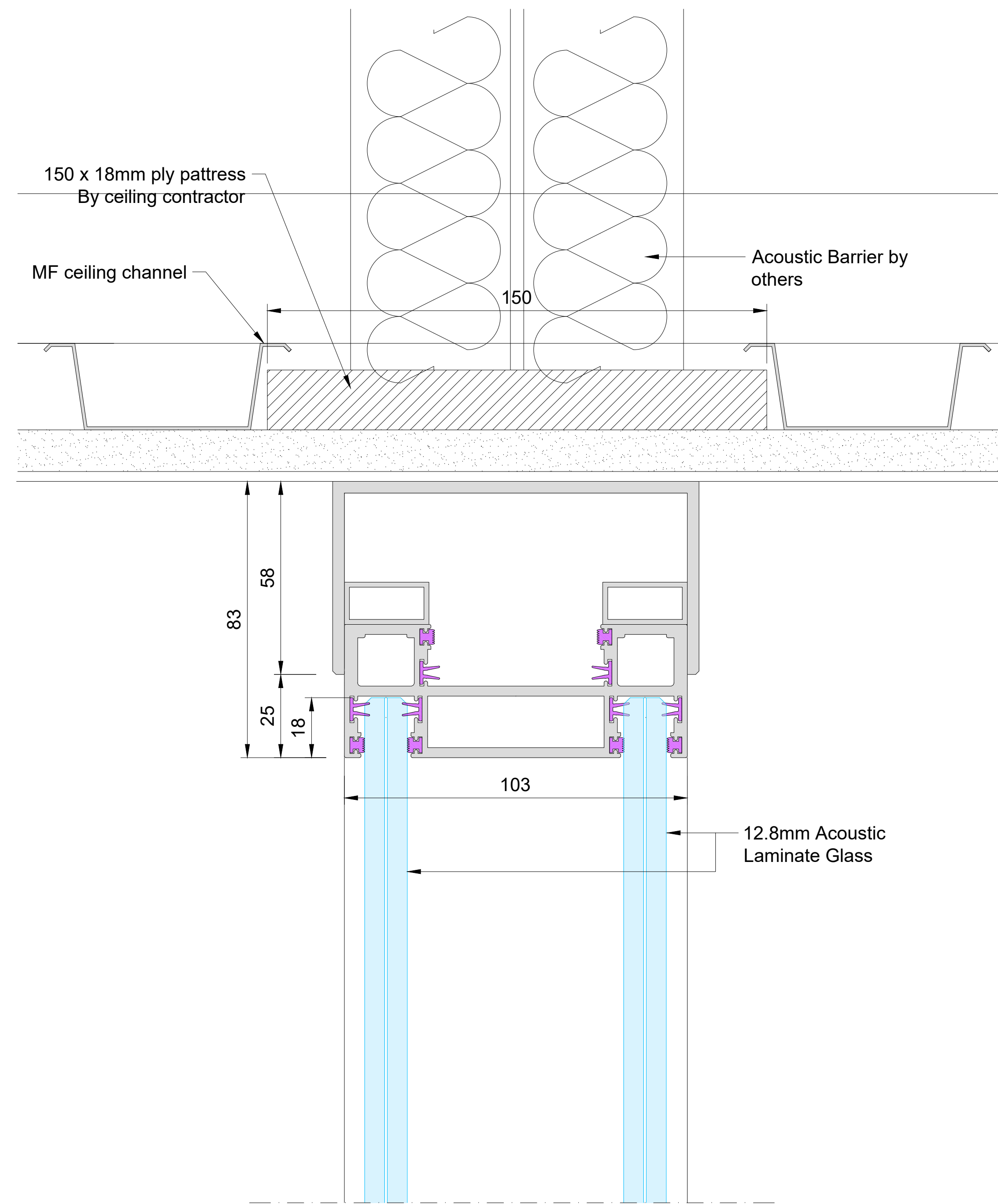
OPTION 1 Surface Mounted Deflection +/- 25mm
