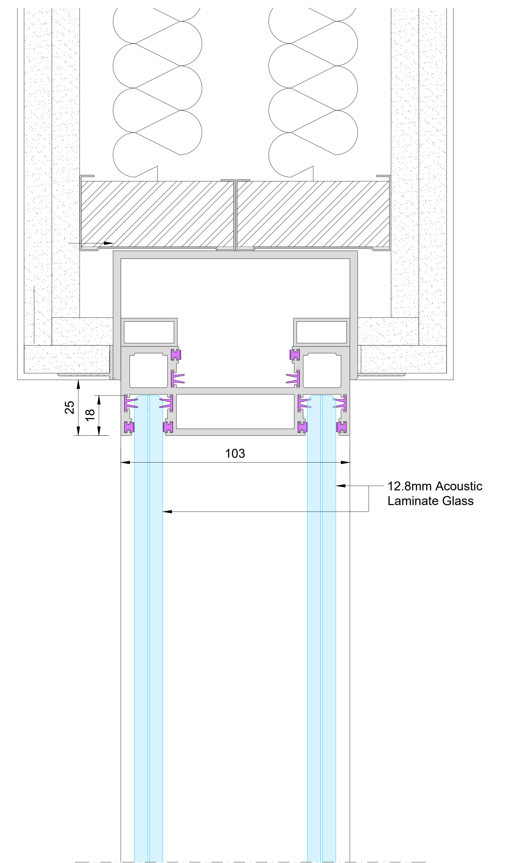
OPTION 3 Recessed Deflection in Bulkhead +/- 25mm
