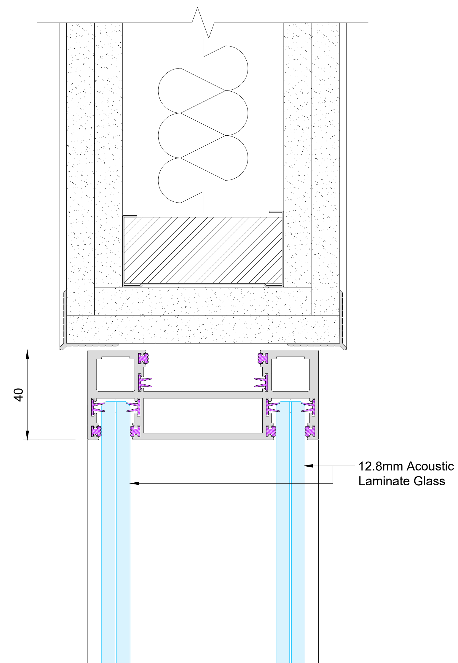
FAIREND ABUTMENT OPTION 1 Surface Mounted Abutment to Drywall Fairend
