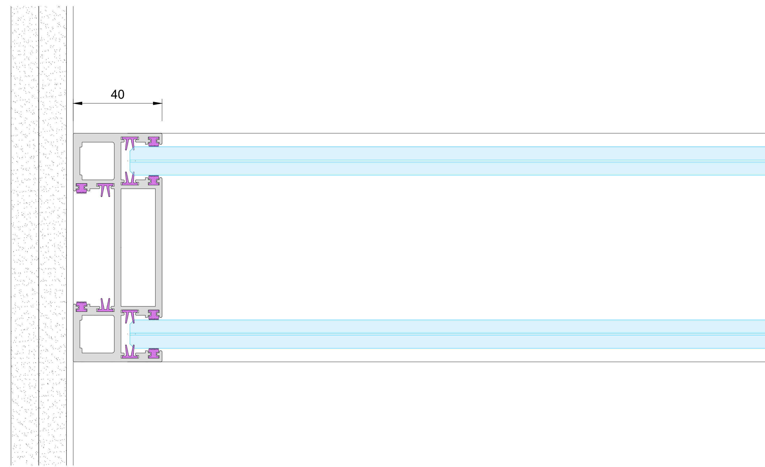
OPTION 1 40mm Abutment
