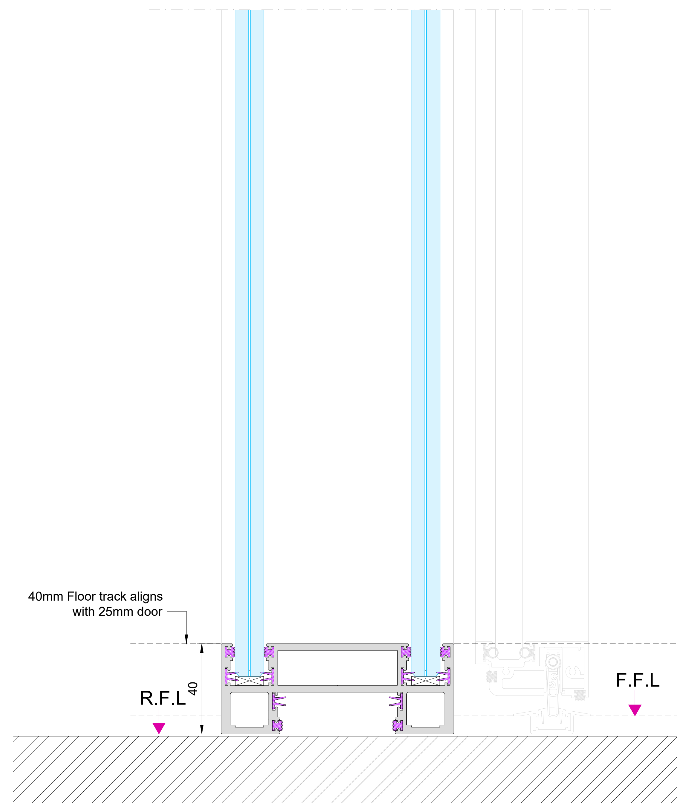
OPTION 1 40mm Base Track
