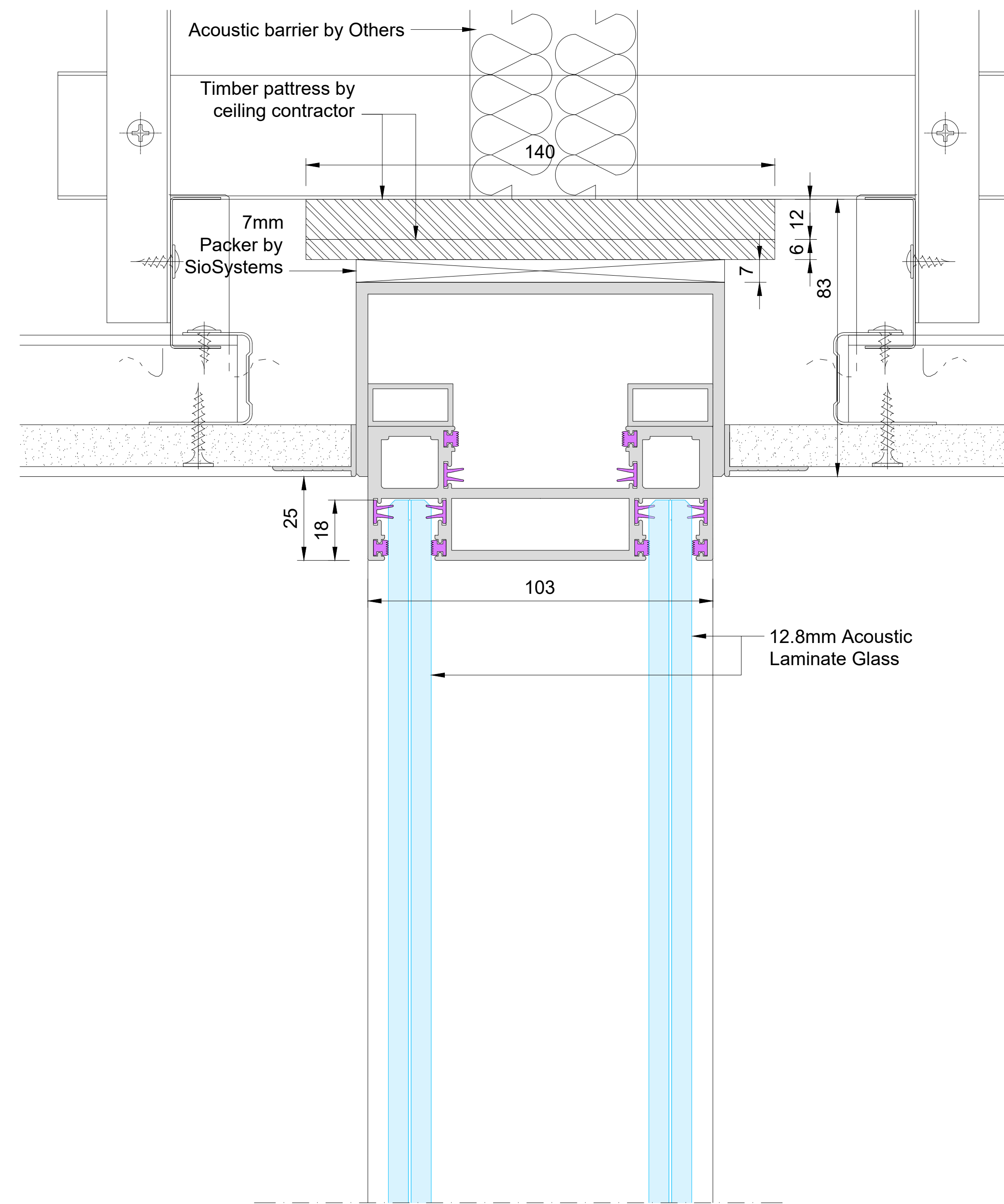
OPTION 2 Recessed Deflection in Ceiling +/- 25mm
