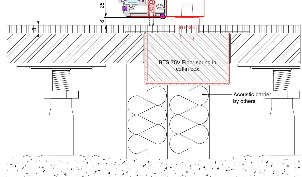
VERTICAL SECTION B:B FULCRUM Single Glazed Pivot Door +/- 25mm Deflection Scale 1:2 @ A0 Acoustic Integrity: 34dB Rw
