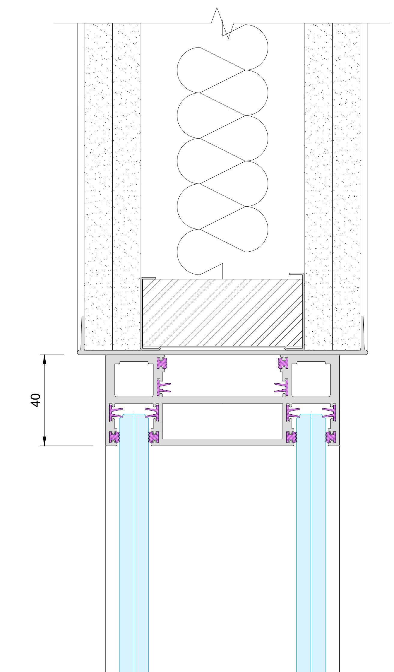
FAIREND ABUTMENT OPTION 2 Surface Mounted Abutment to Drywall Endcap
