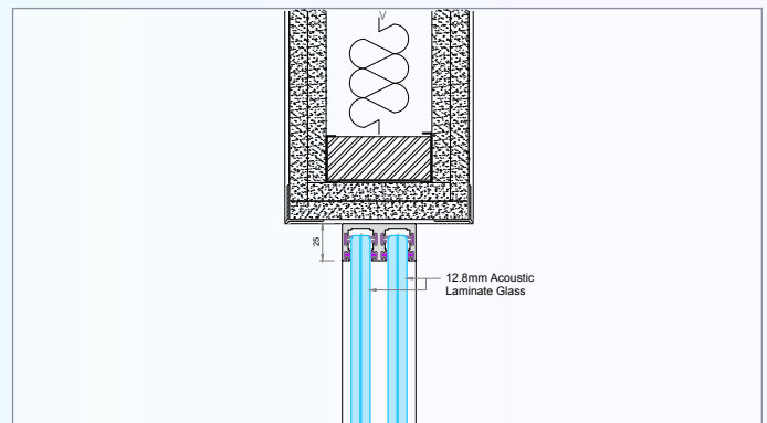
Surface Mouted Abutment to Drywall Fairend
