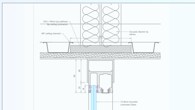
Single Glazed Head Track +/- 25mm Deflection
