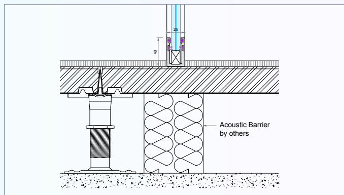
Single Glazed Floor Track
