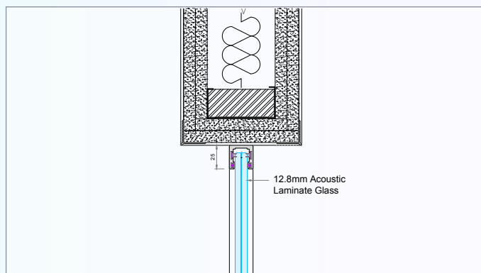
Surface Mounted Abutment to Drywall Fairend
