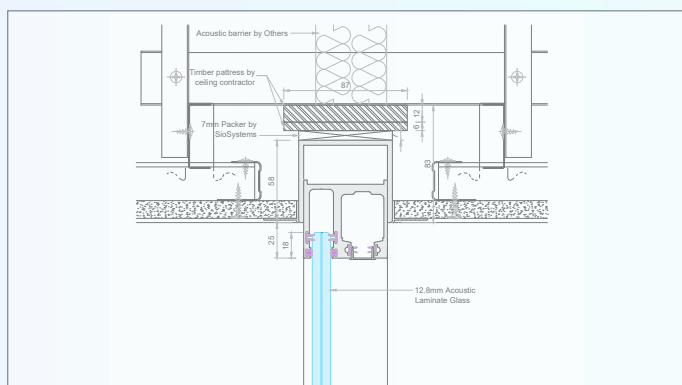
Recessed Deflection in Ceiling +/- 25mm
