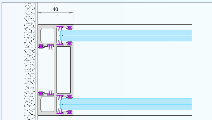
40mm Abutment
