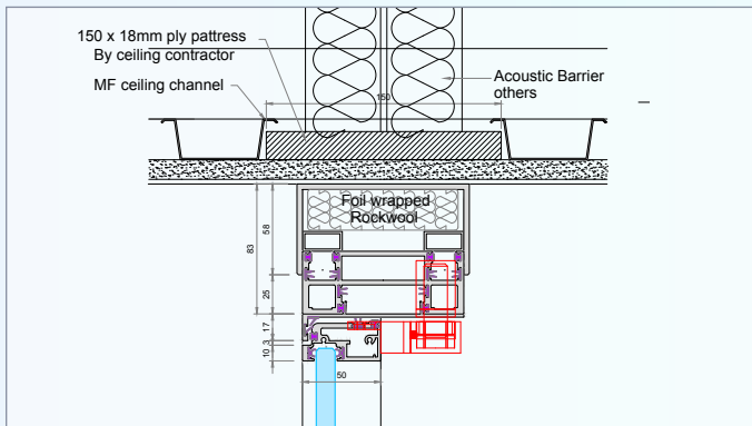
Single Glazed Pivot Door +/- 25mm Deflection
