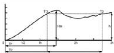
Dough Development Curve
