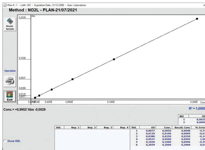
Calibration curve
