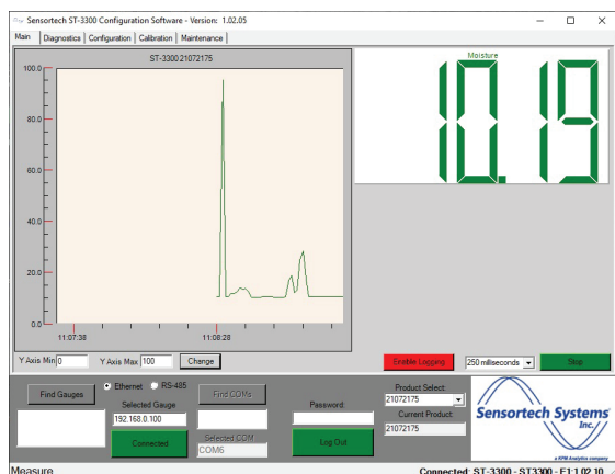
PC interface
