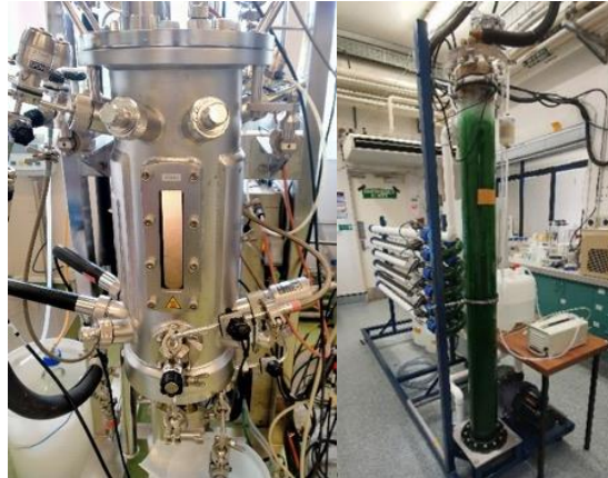
Figure 2: Left, 10 L fermentation bioreactor growing the extremophilic methanotroph (bacterium) at BSI-Scion Group. Right, 80 L photobioreactor growing the extremophilic microalga at University of Canterbury.
