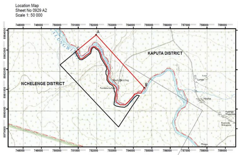
Map 12: Location of Site for Mini Hydro Power Plant at Kundabwika Falls
