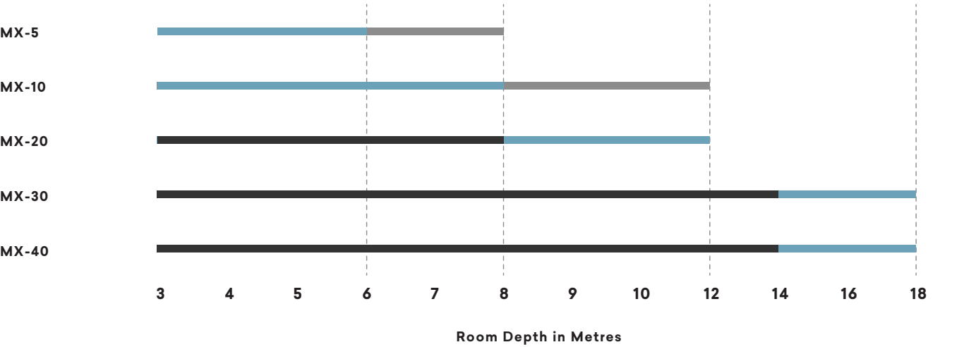
Series MX SPL Performance
