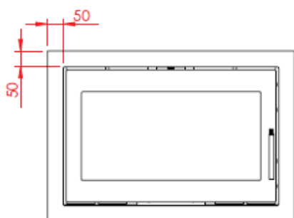
470 XL IR, airbox behind
