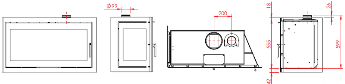
550 XXL fixed glass 1 side, airbox on top
