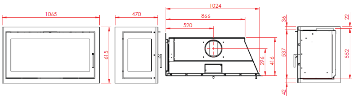
550 XXL fixed glass 1 side, airbox behind
