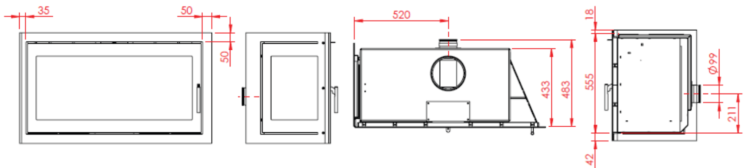
550 XXL fixed glass 1 side, airbox behind
