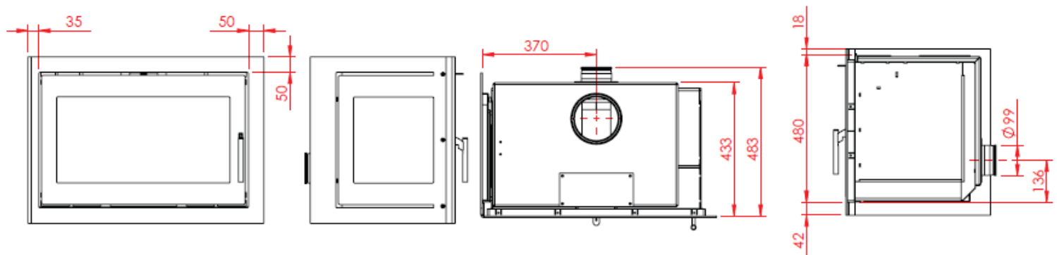
470 XL fixed glass 1 side, airbox behind
