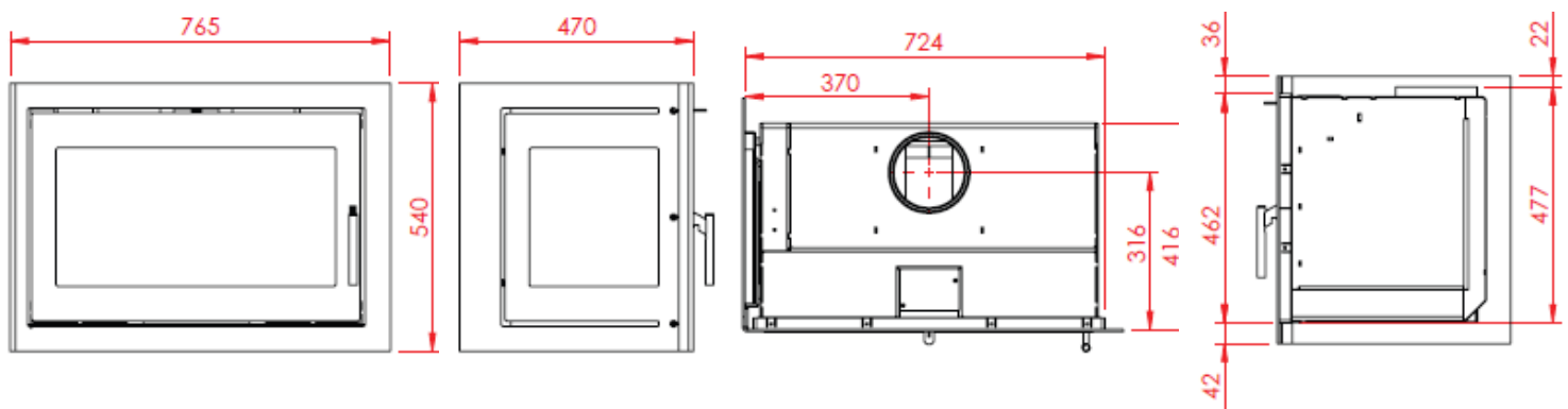
470 XL fixed glass 1 side
