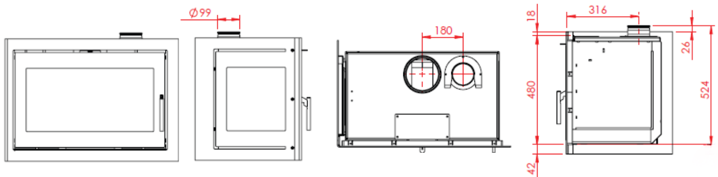
470 XL fixed glass 1 side, airbox on top
