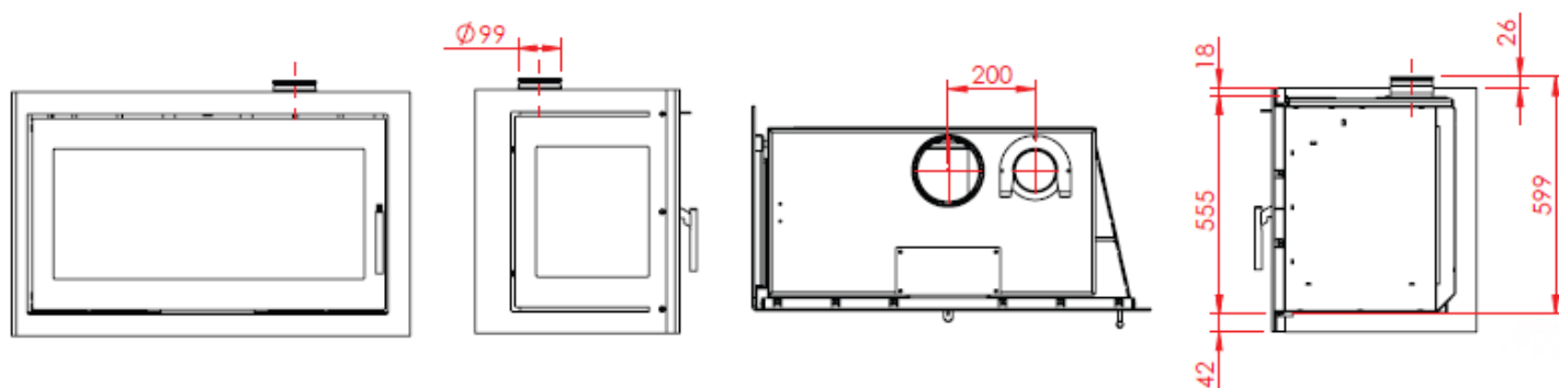
550-850 fixed glass 1 side, airbox on top
