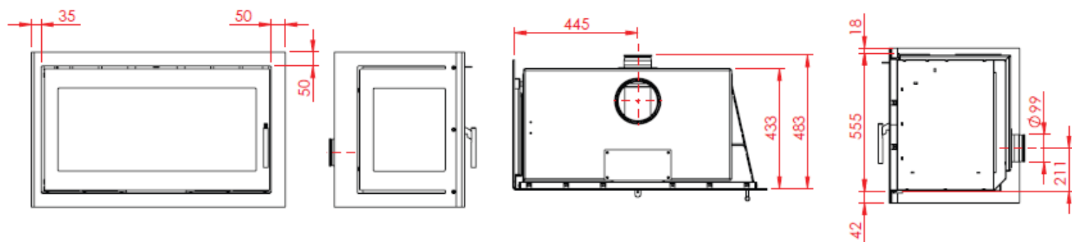
550-850 fixed glass 1 side, airbox behind
