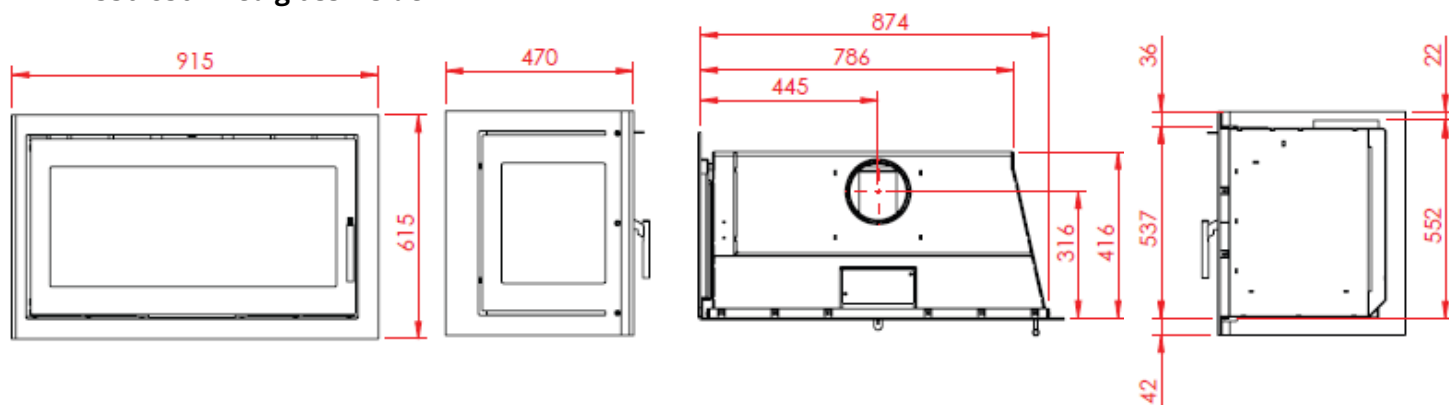
550-850 fixed glass 1 side
