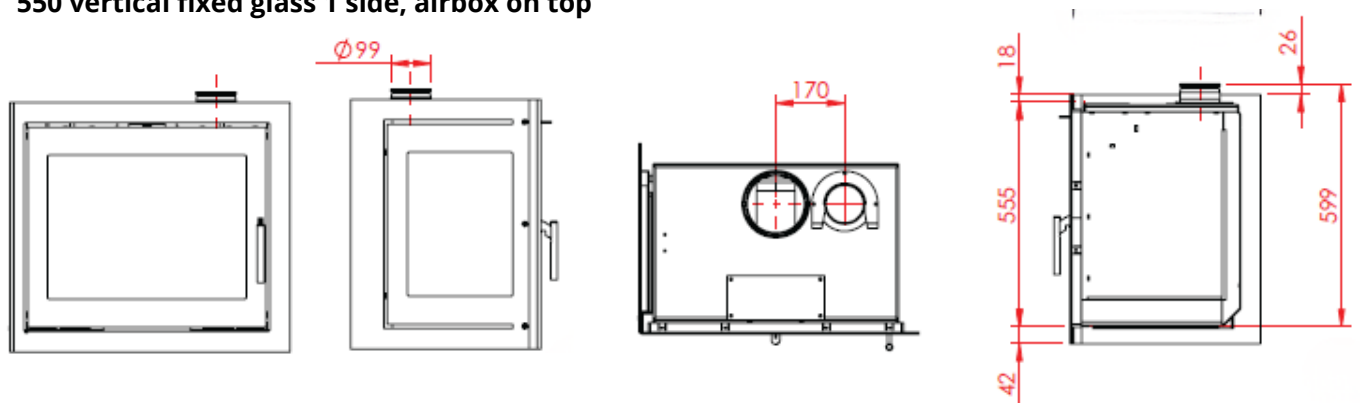
550 vertical fixed glass 1 side, airbox on top
