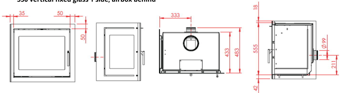
550 vertical fixed glass 1 side, airbox behind
