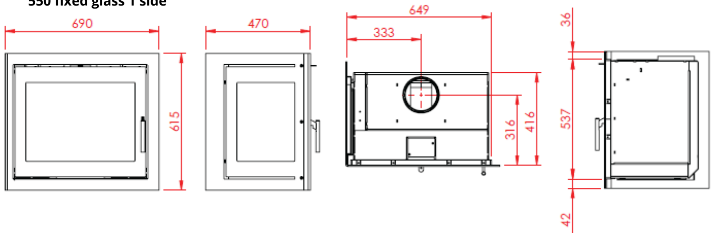
550 vertical fixed glass 1 side, airbox behind
