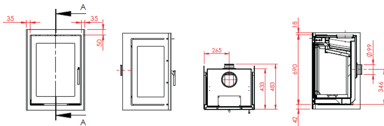
550 vertical fixed glass 2 sides, airbox on top
