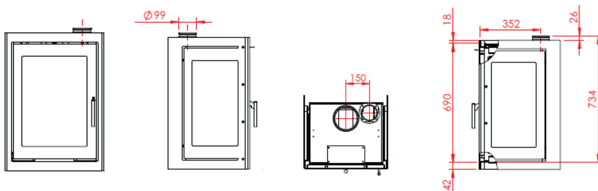
550 vertical fixed glass 2 sides, airbox on top
