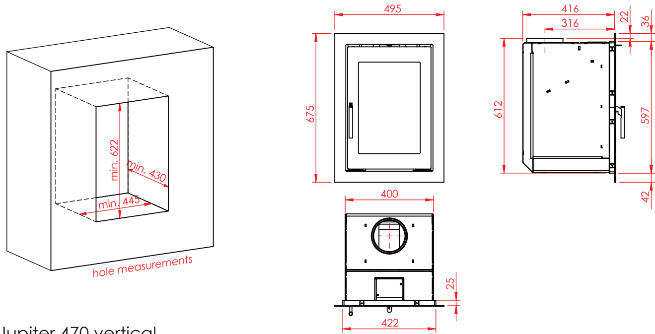
Jupiter 470 vertical
