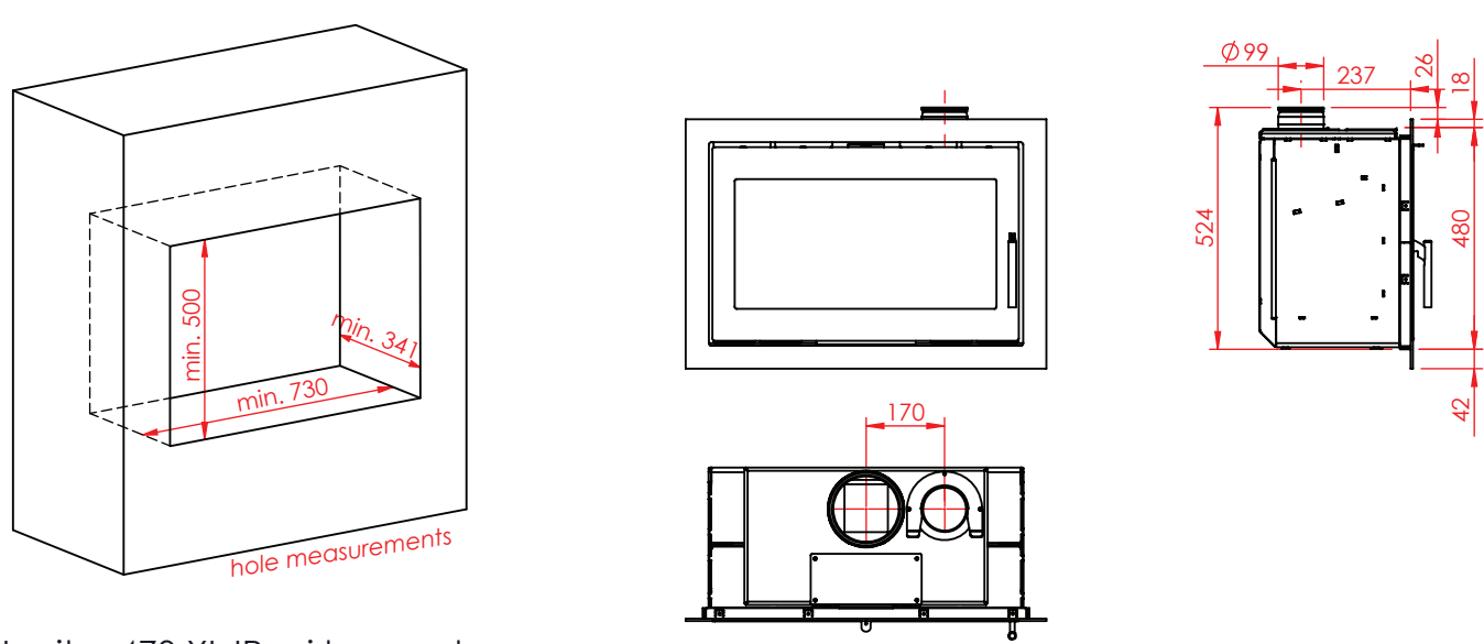
Jupiter 470 XL IR, airbox on top
