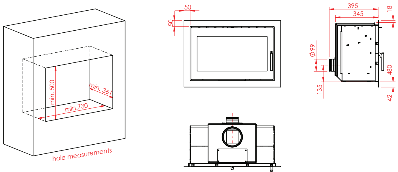
Jupiter 470 XL IR, airbox behind
