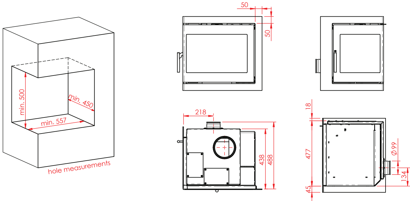
Jupiter 470 with angular door, airbox side
