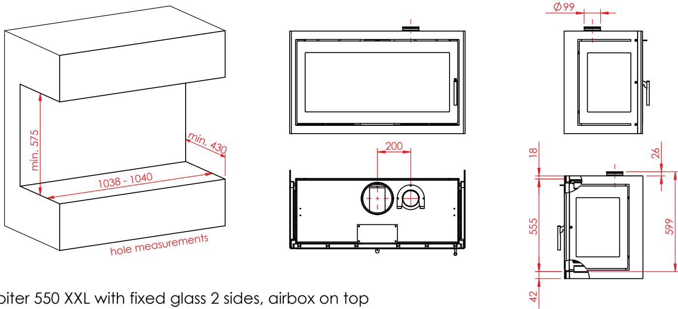
Jupiter 550 XXL with fixed glass 2 sides
