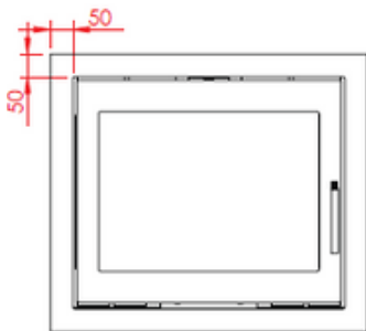
550 with curved door, airbox behind
