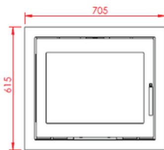
550 with curved door
