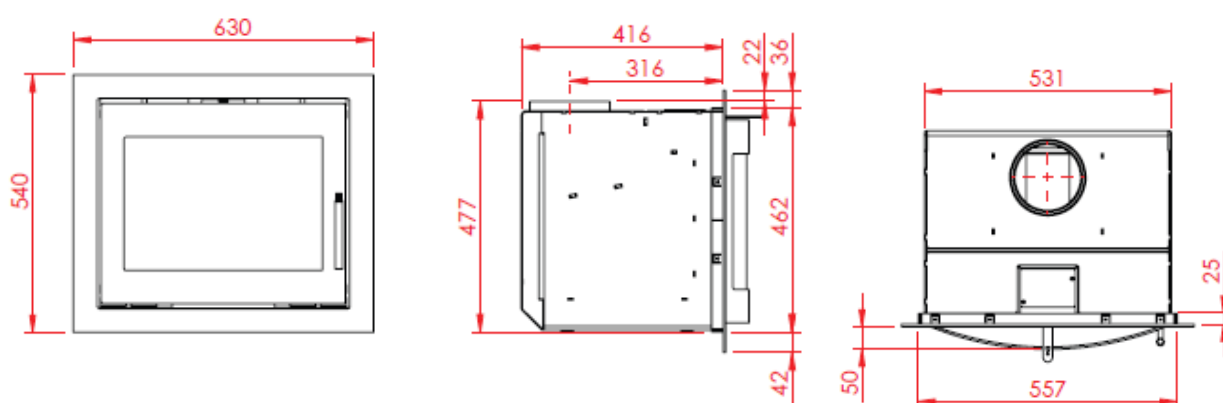
470 with curved door, airbox behind
