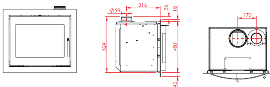
470 with curved door, airbox on top
