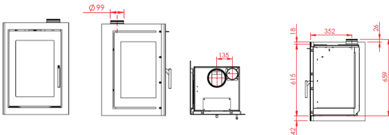
470 vertical fixed glass 1 side, airbox on top
