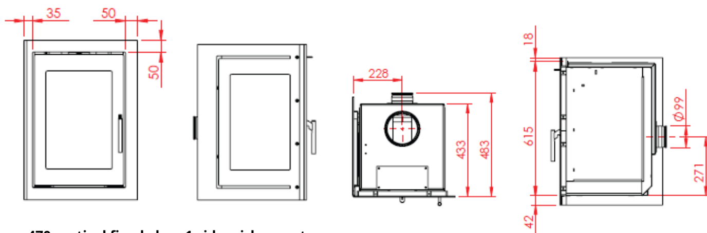
470 vertical fixed glass 1 side, airbox on top
