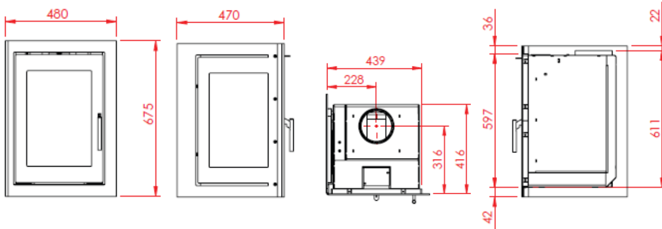
470 vertical fixed glass 1 side, airbox behind
