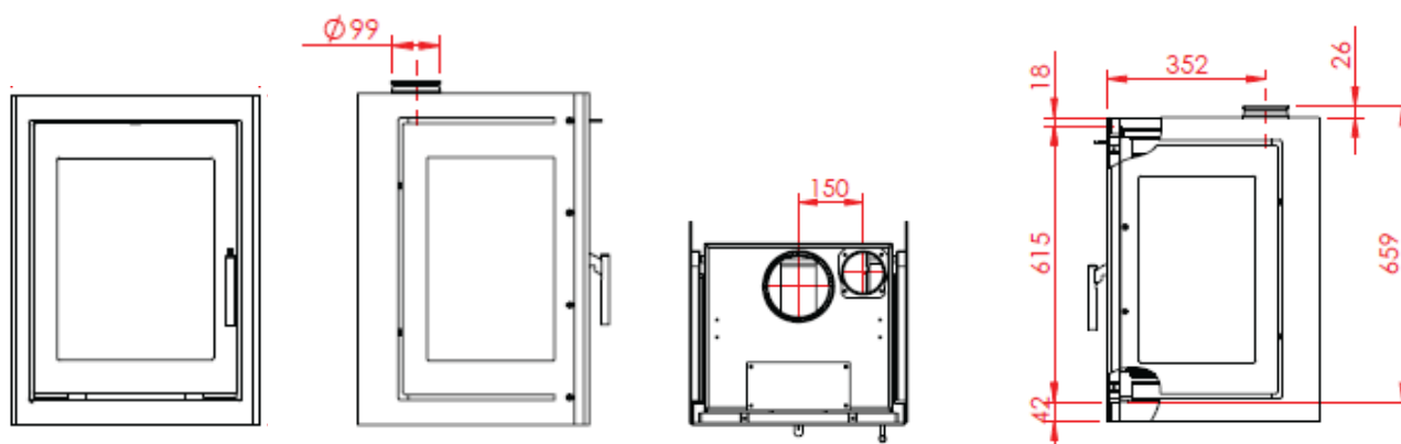
470 vertical fixed glass 2 sides, airbox on top
