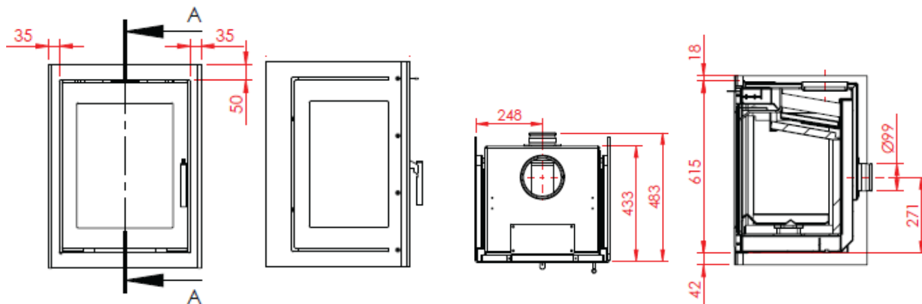
470 vertical fixed glass 2 sides, airbox behind
