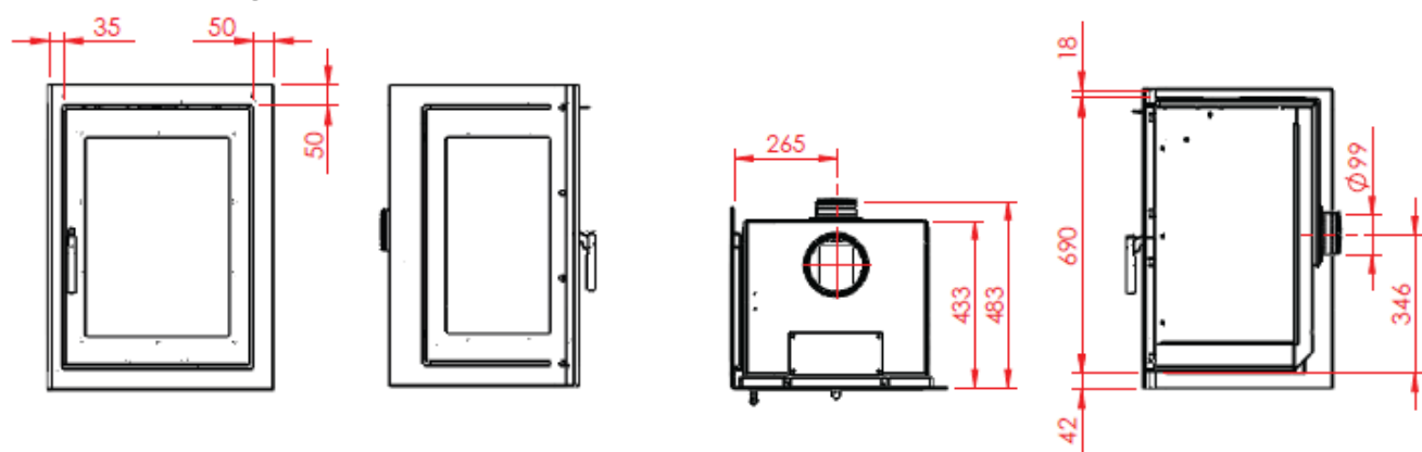
550 vertical fixed glass 1 side, airbox behind
