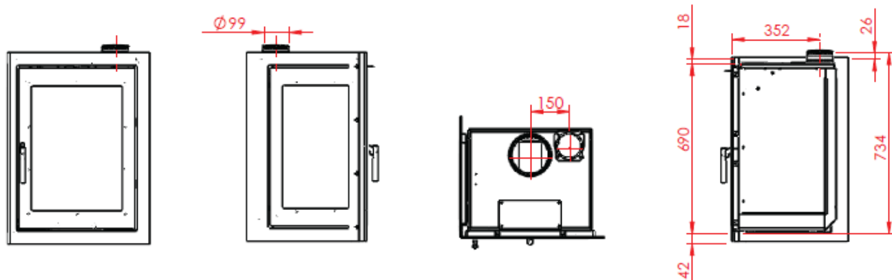
550 vertical fixed glass 1 side, airbox on top
