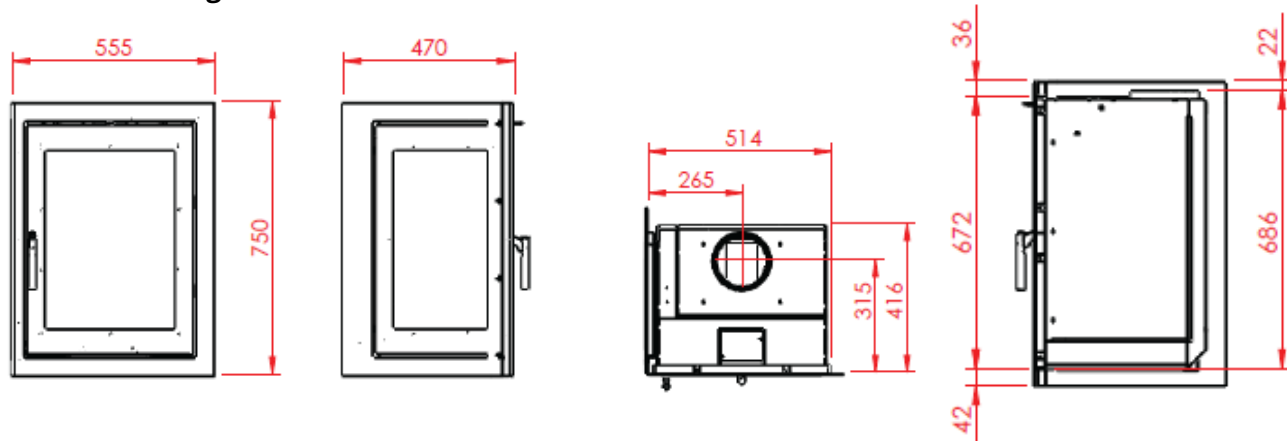
550 vertical fixed glass 1 side, airbox behind
