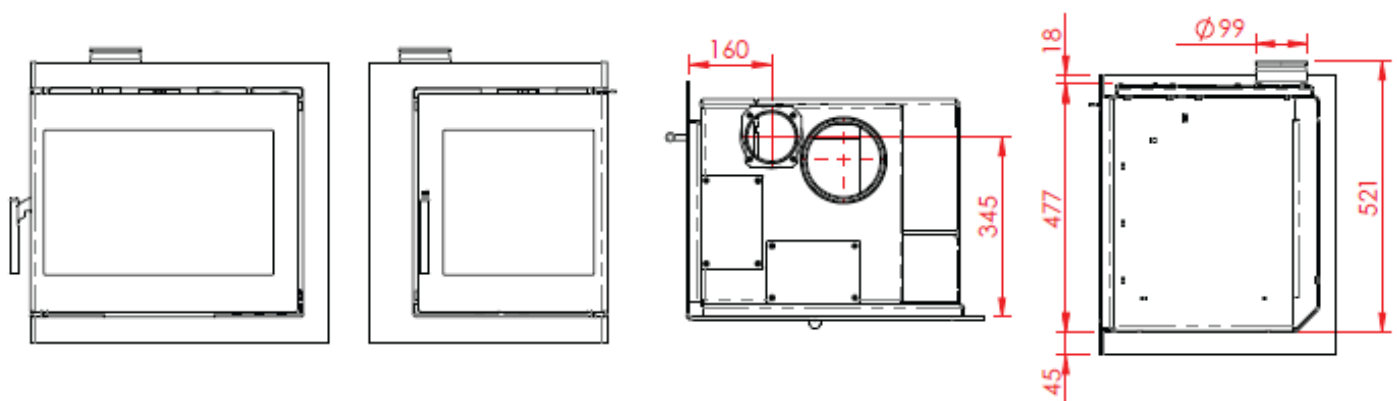
470 with angular door, airbox on top
