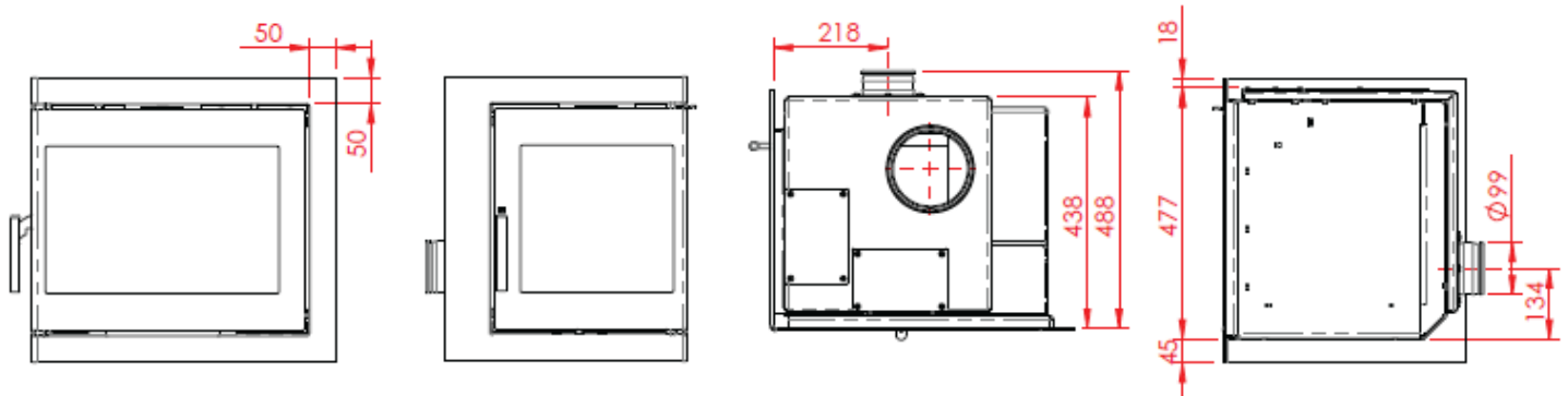
470 with angular door, airbox behind
