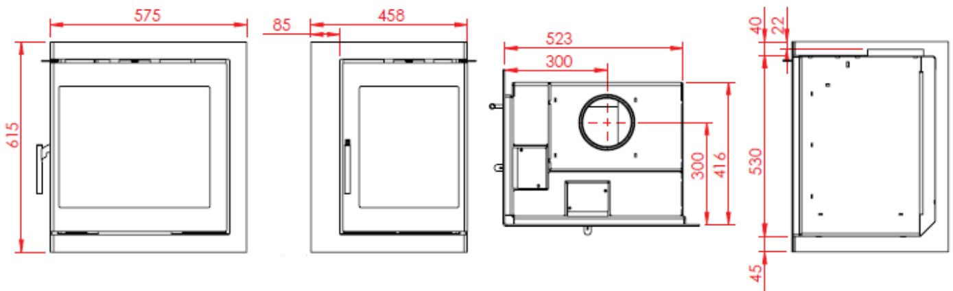
550 with angular door, airbox behind
