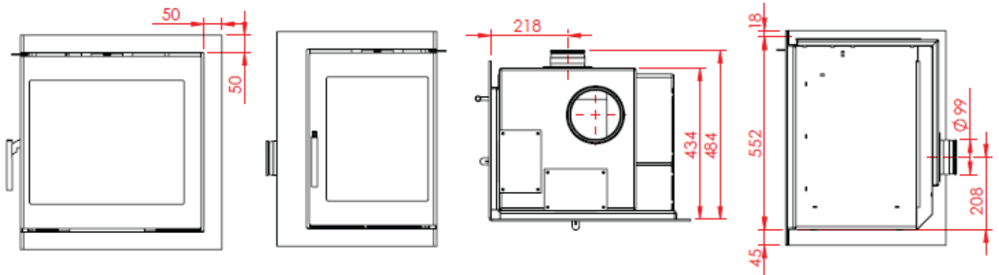
550 with angular door, airbox behind
