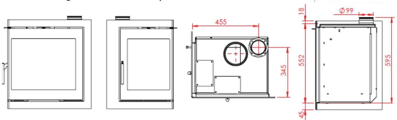
550 with angular door, airbox on top
