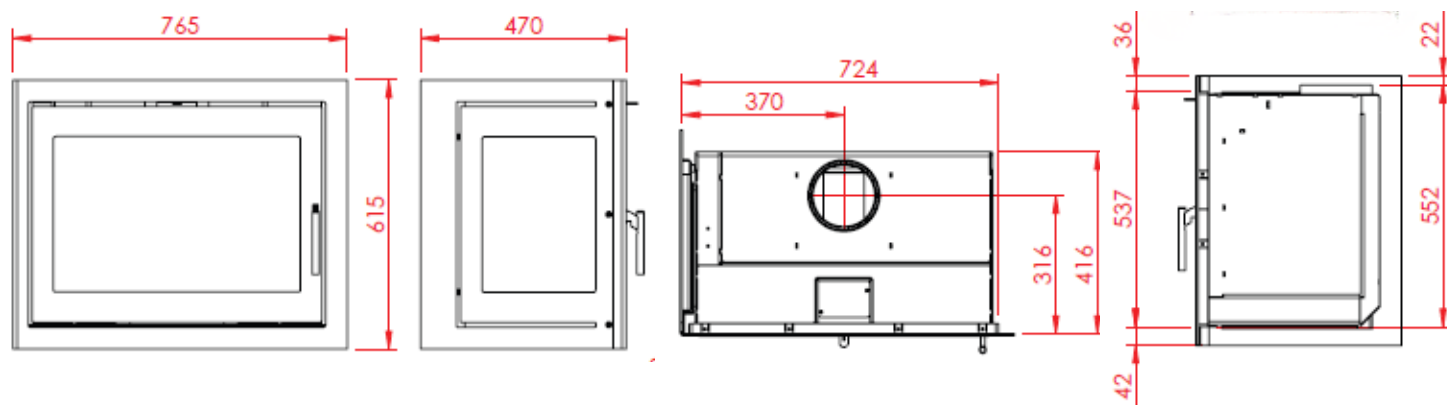
550 XL fixed glass 1 side, airbox behind
