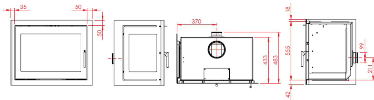
550 XL fixed glass 1 side, airbox on top
