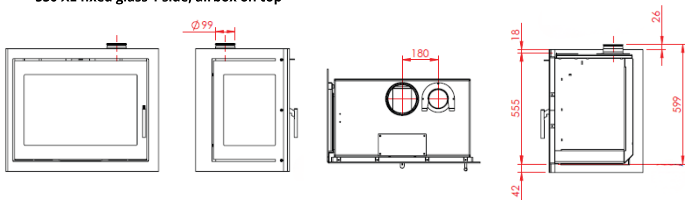
550 XL fixed glass 1 side, airbox on top
