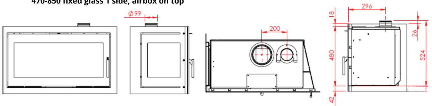
470-850 fixed glass 1 side, airbox on top
