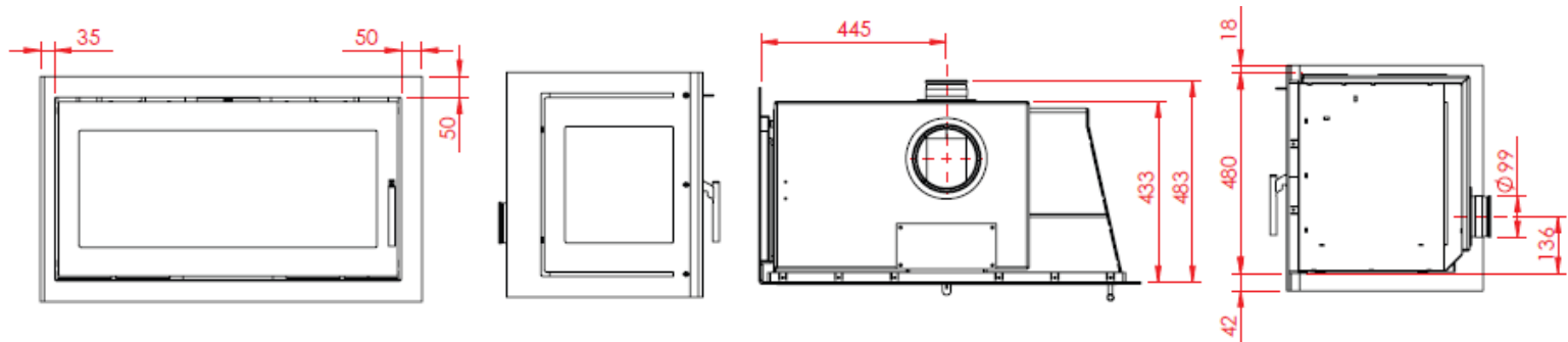
470-850 fixed glass 1 side, airbox behind
