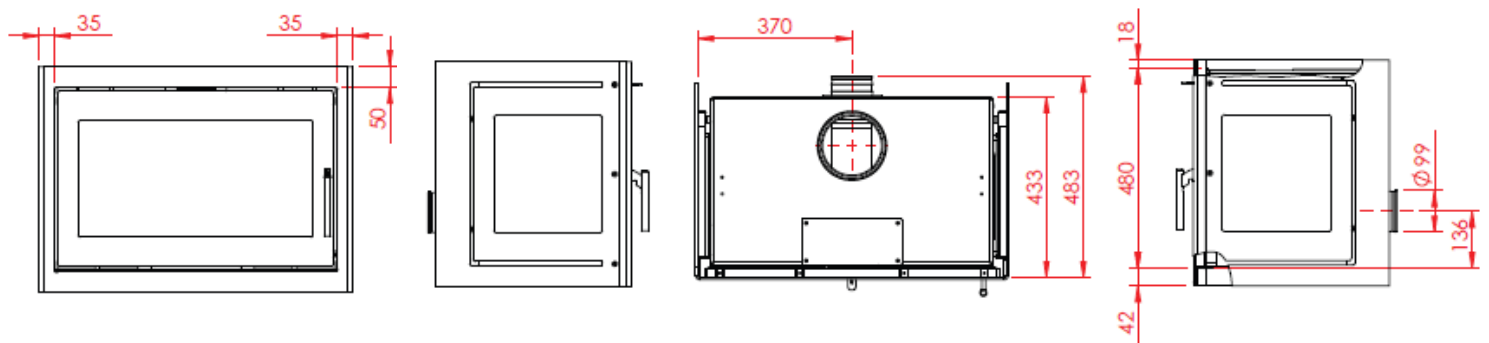
470 XL fixed glass 2 sides, airbox behind
