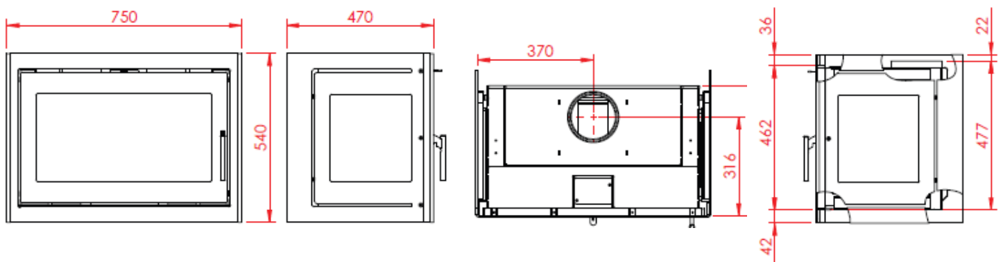
470 XL fixed glass 2 sides, airbox behind
