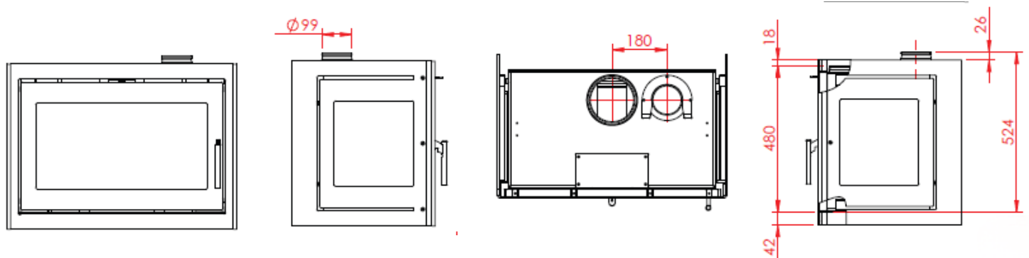
470 XL fixed glass 2 sides, airbox on top
