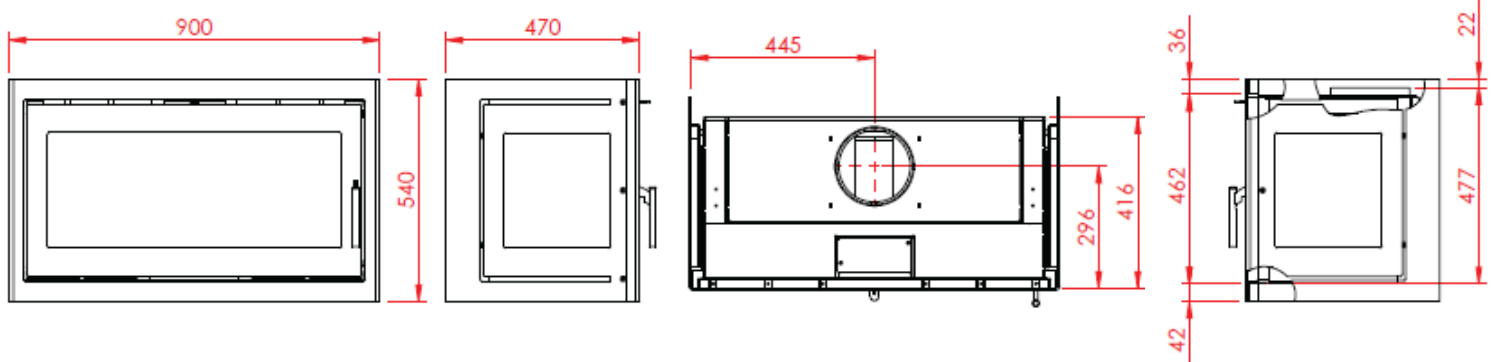
470-850 fixed glass 2 sides
