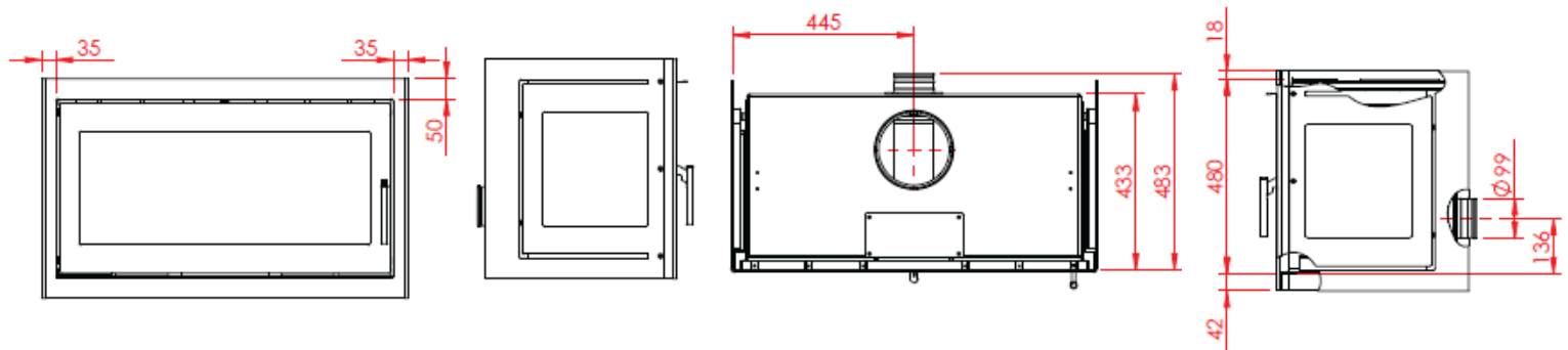
470-850 fixed glass 2 sides, airbox behind
