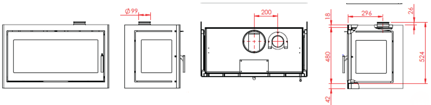
470-850 fixed glass 2 sides, airbox on top
