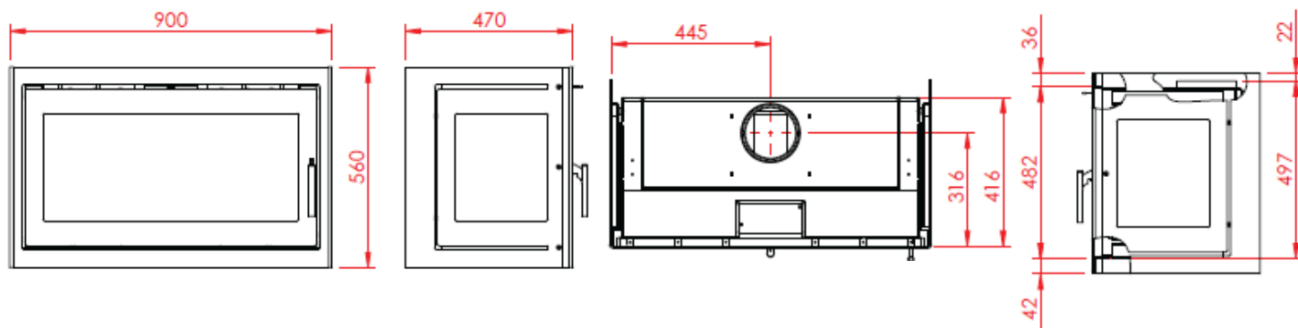
500-850 fixed glass 2 sides
