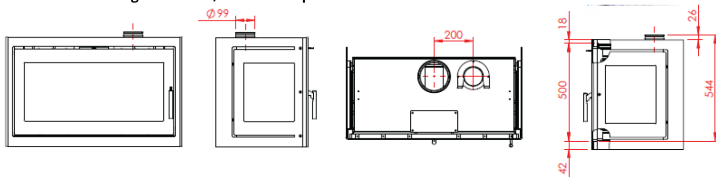
500-850 fixed glass 2 sides, airbox on top
