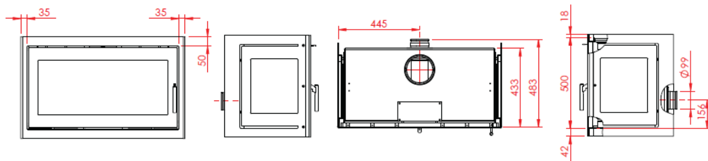
500-850 fixed glass 2 sides, airbox behind
